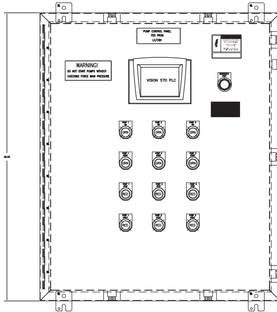
PUMP_CONTROL_PANEL 36"W x 30"H x 107"D FRONT VIEW OUTER DOOR
