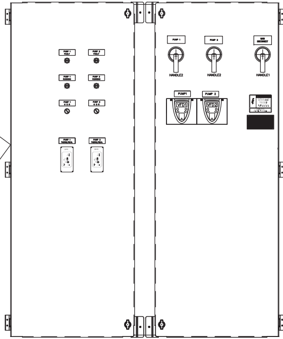
FRONT VIEW INNER SWING PANELS
