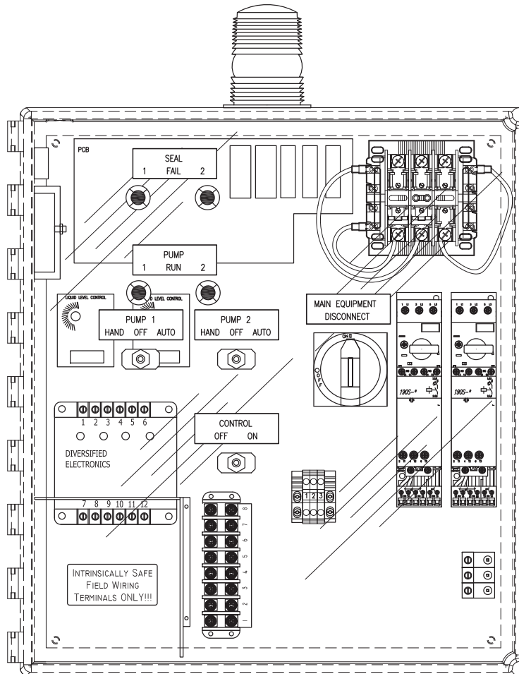
24 x 24 x 10 ENCLOSURE WITH OUTER DOOR REMOVED LEXAN INNER DOOR
