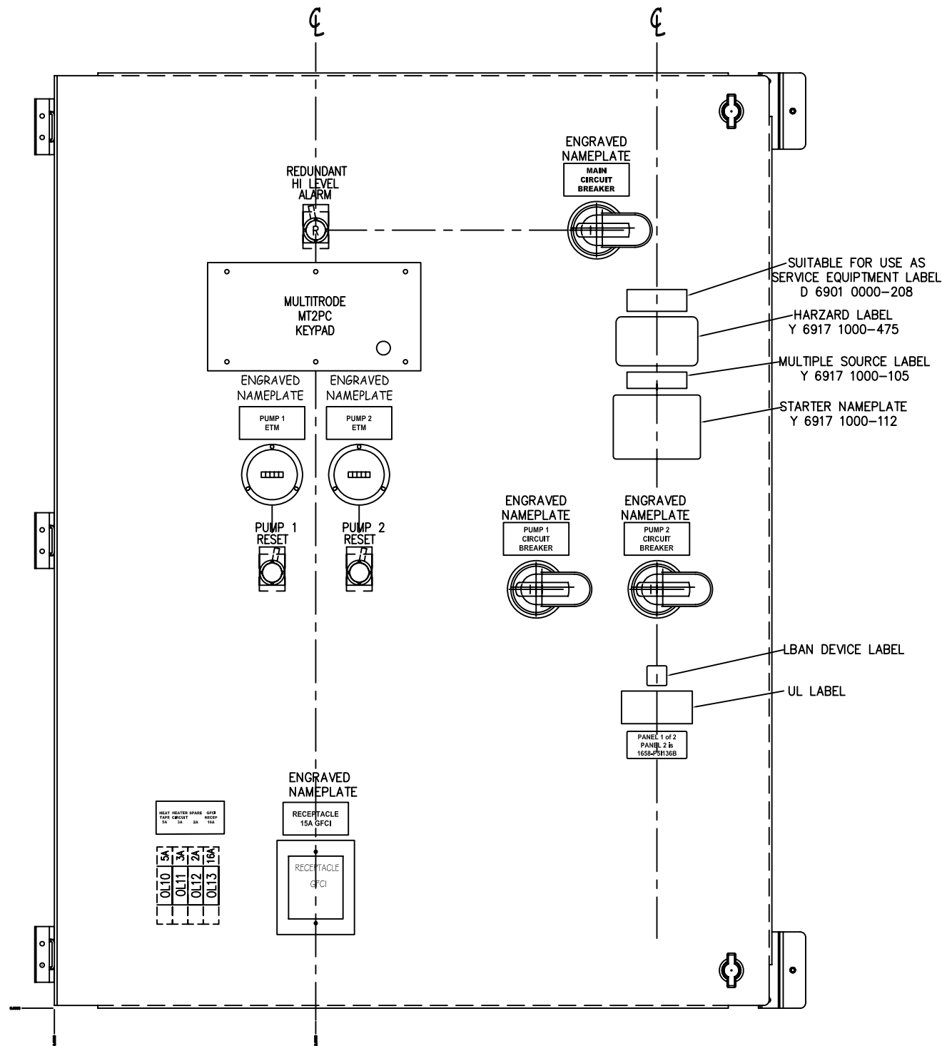
FRONT VIEW 33" X 43" SWING PANEL
