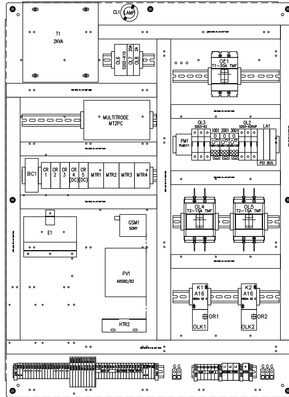
FRONT VIEW 33" X 45" SUB-PANEL
