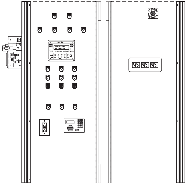
FRONT VIEW SWING PANELS (OUTER DOORS REMOVED)
