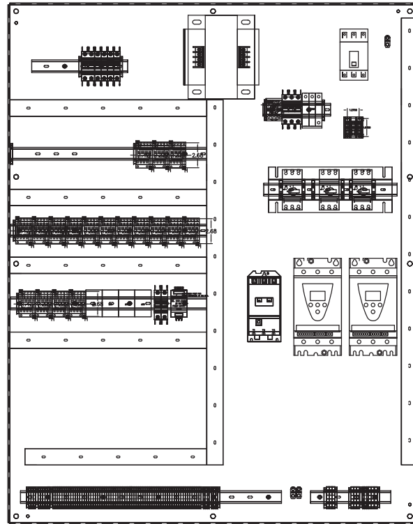
FRONT VIEW PANEL (DOOR/SWING OUT PANEL REMOVED)
