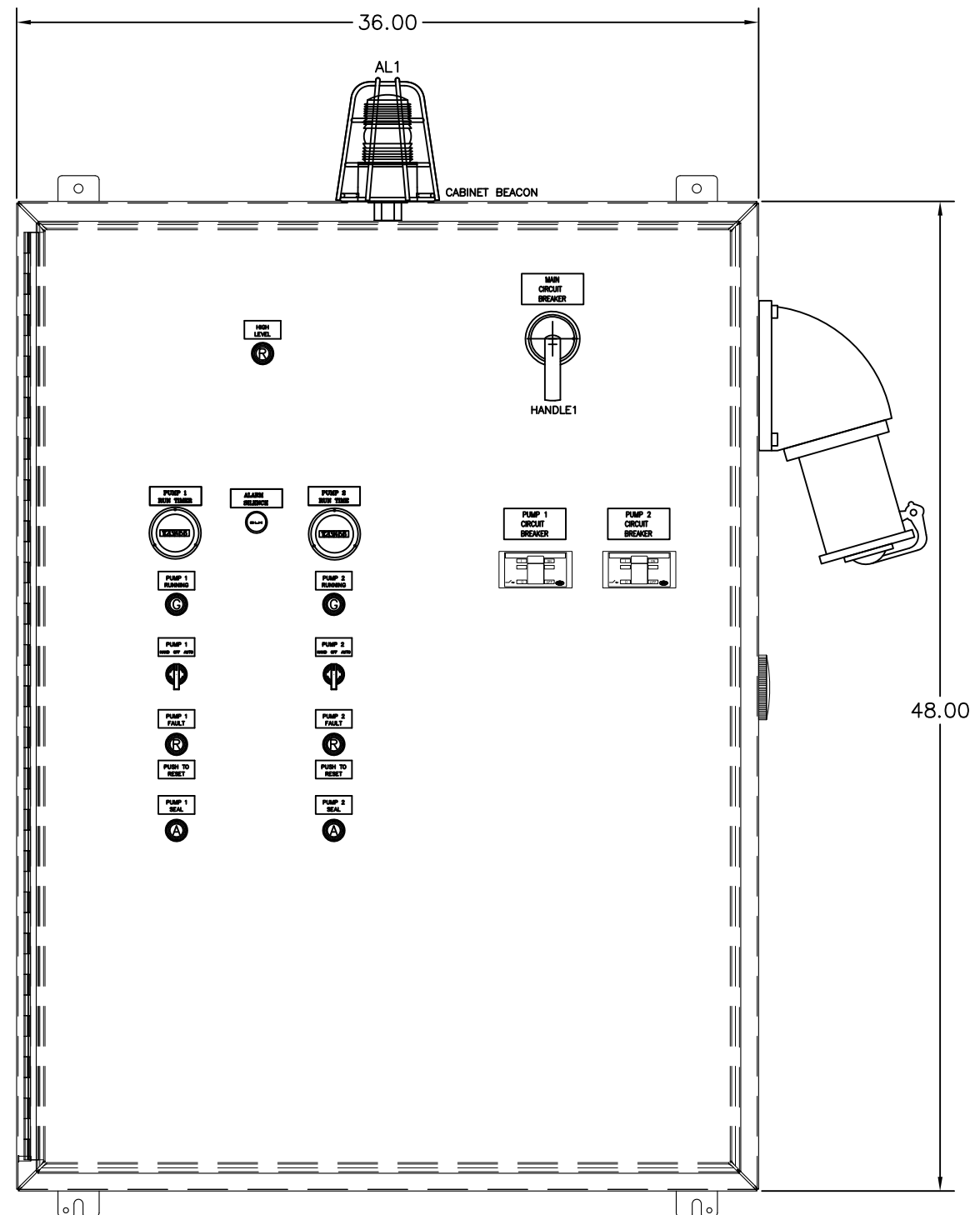
FRONT VIEW
