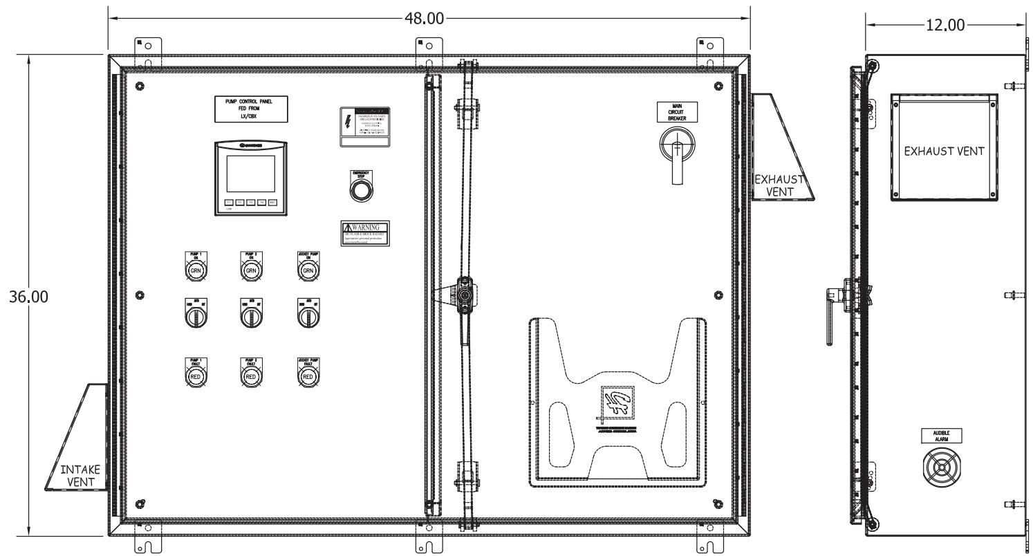
PUMP CONTROL PANEL NEMA 12 36"X48"X12"
