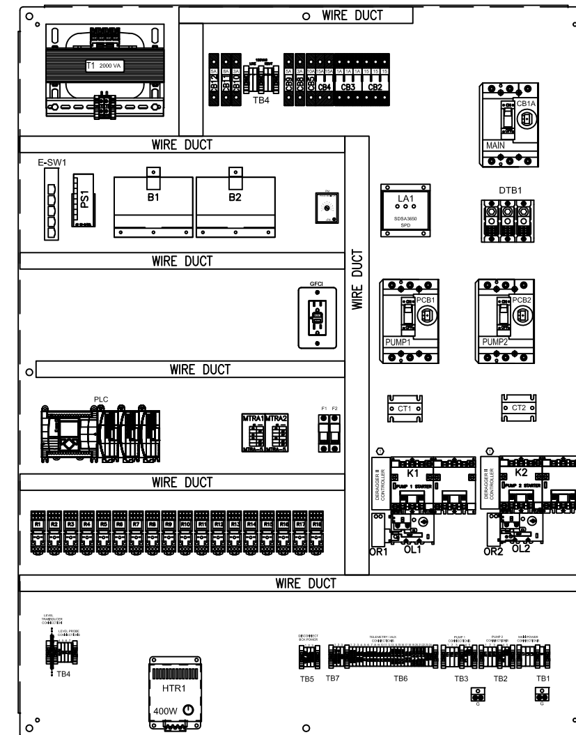
FRONT VIEW SUBPANEL
