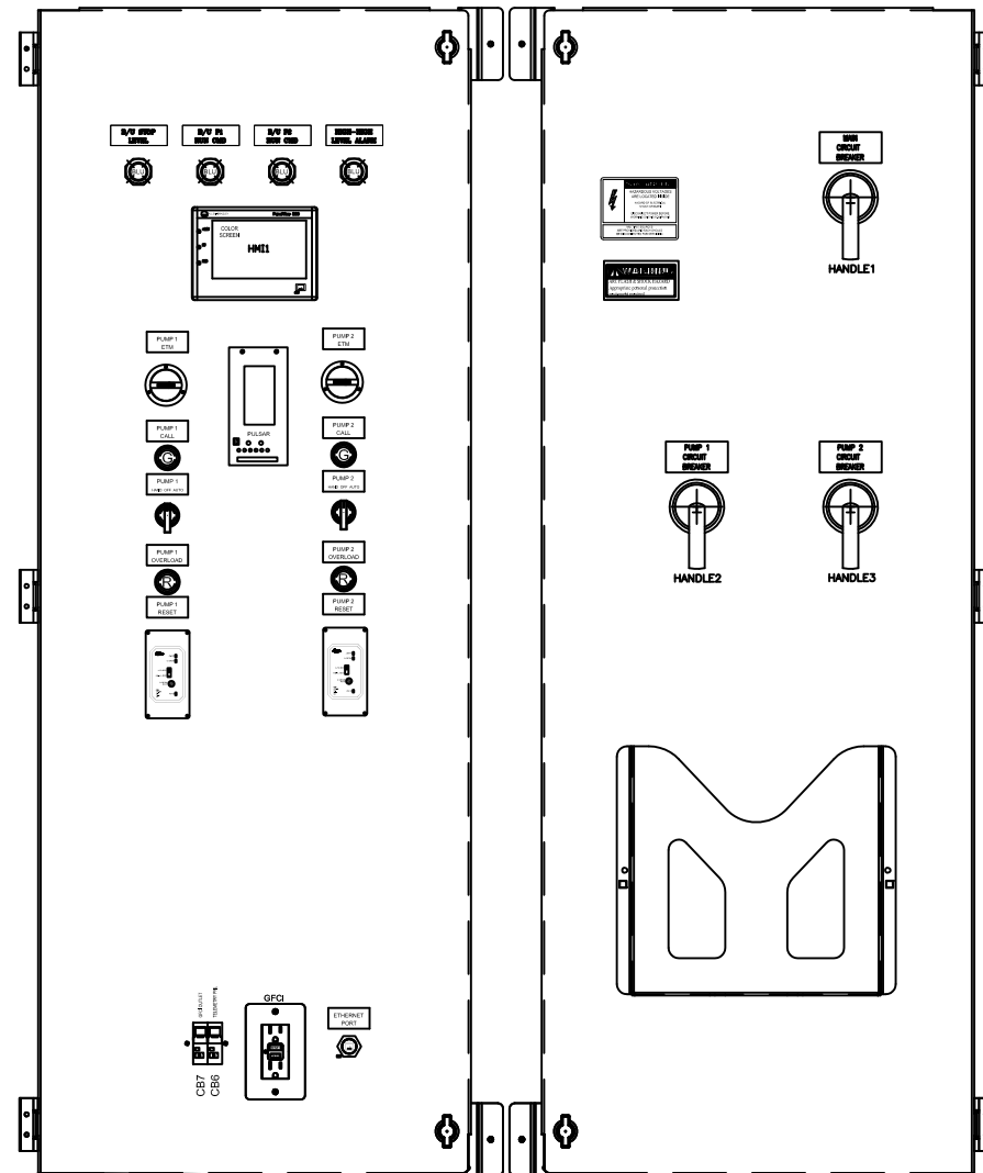
FRONT VIEW SWING PANELS
