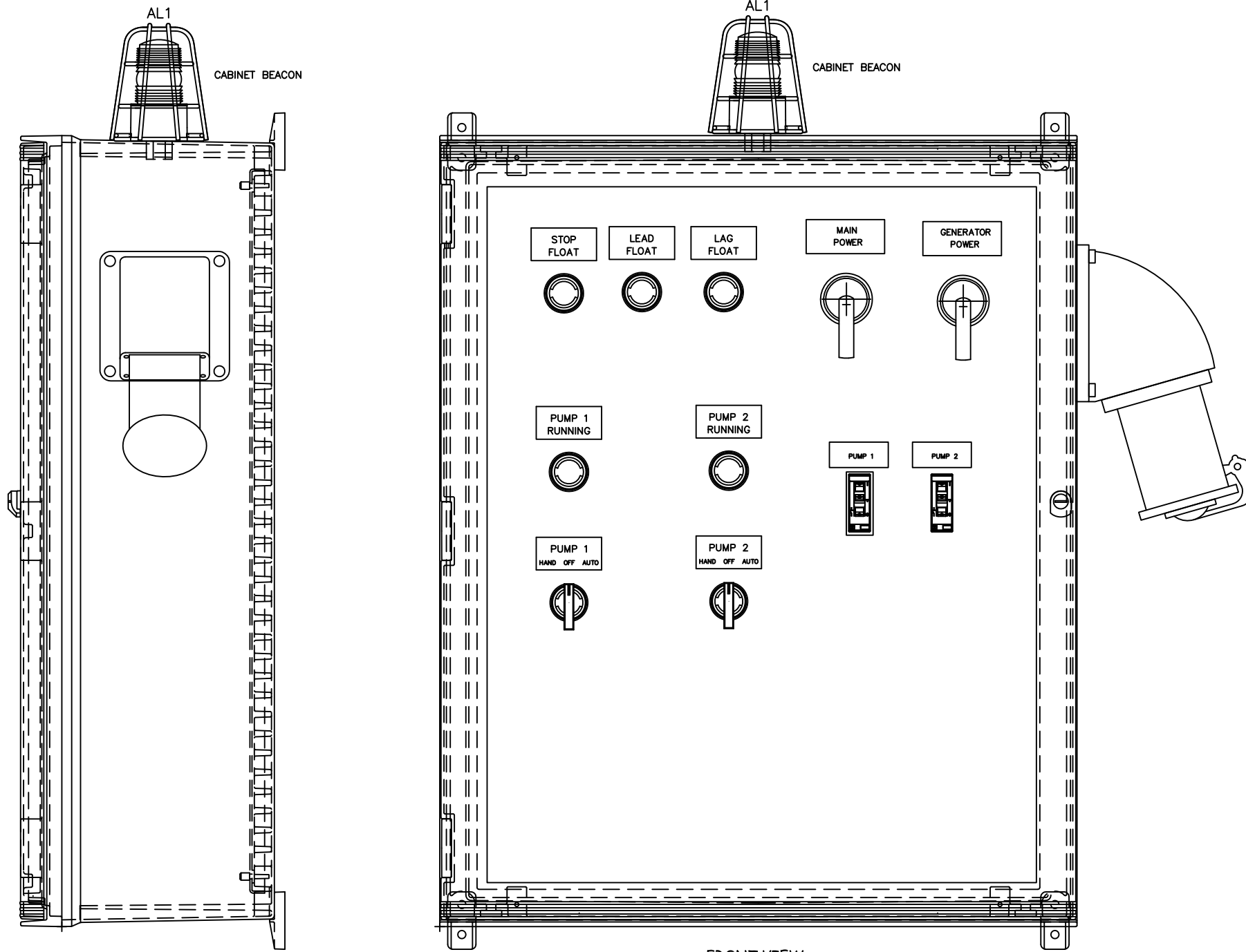
FRONT VIEW INNER DOOR
