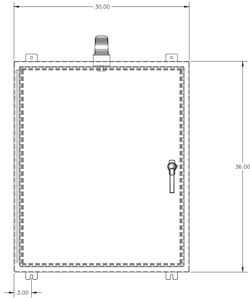
FRONT VIEW
