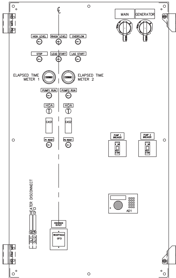
FRONT VIEW SWING PANEL
