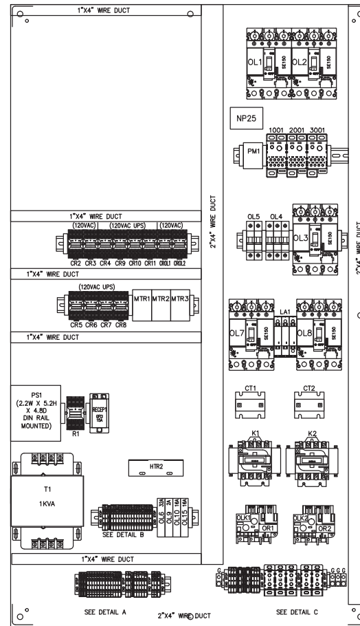
FRONT VIEW SUB-PANEL
