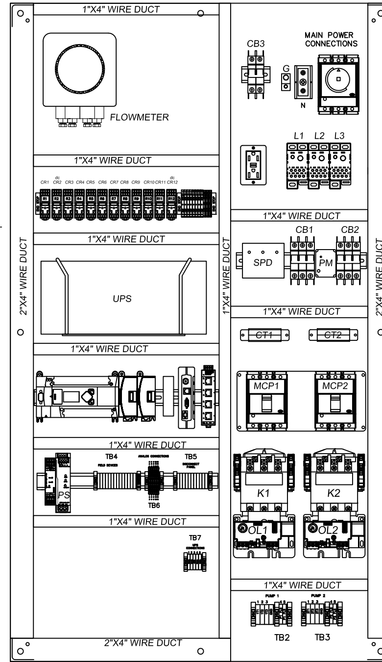
SUB-PANEL FRONT VIEW
