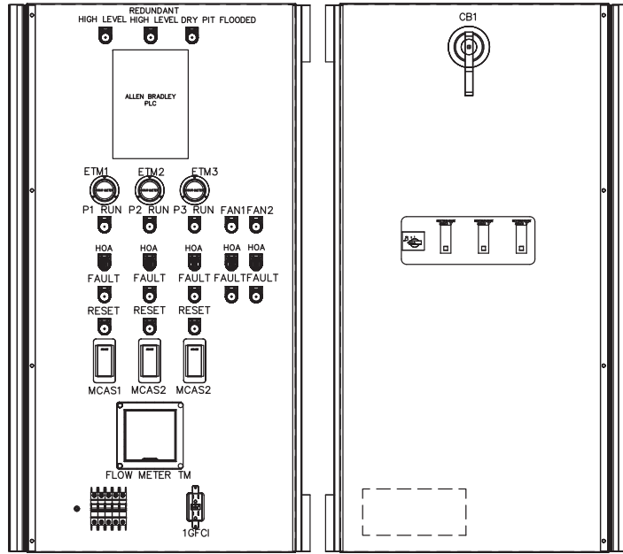
FRONT VIEW SWING PANEL (DOOR REMOVED)
