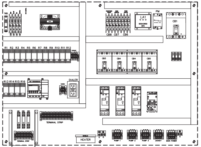
BACKPLATE VIEW
