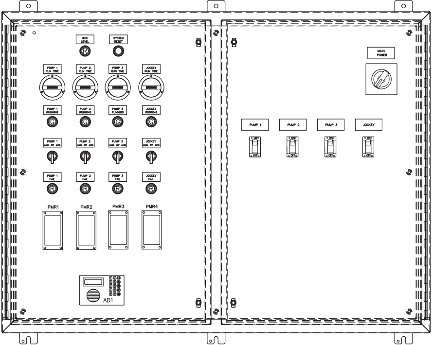
DEADFRONT VIEW
