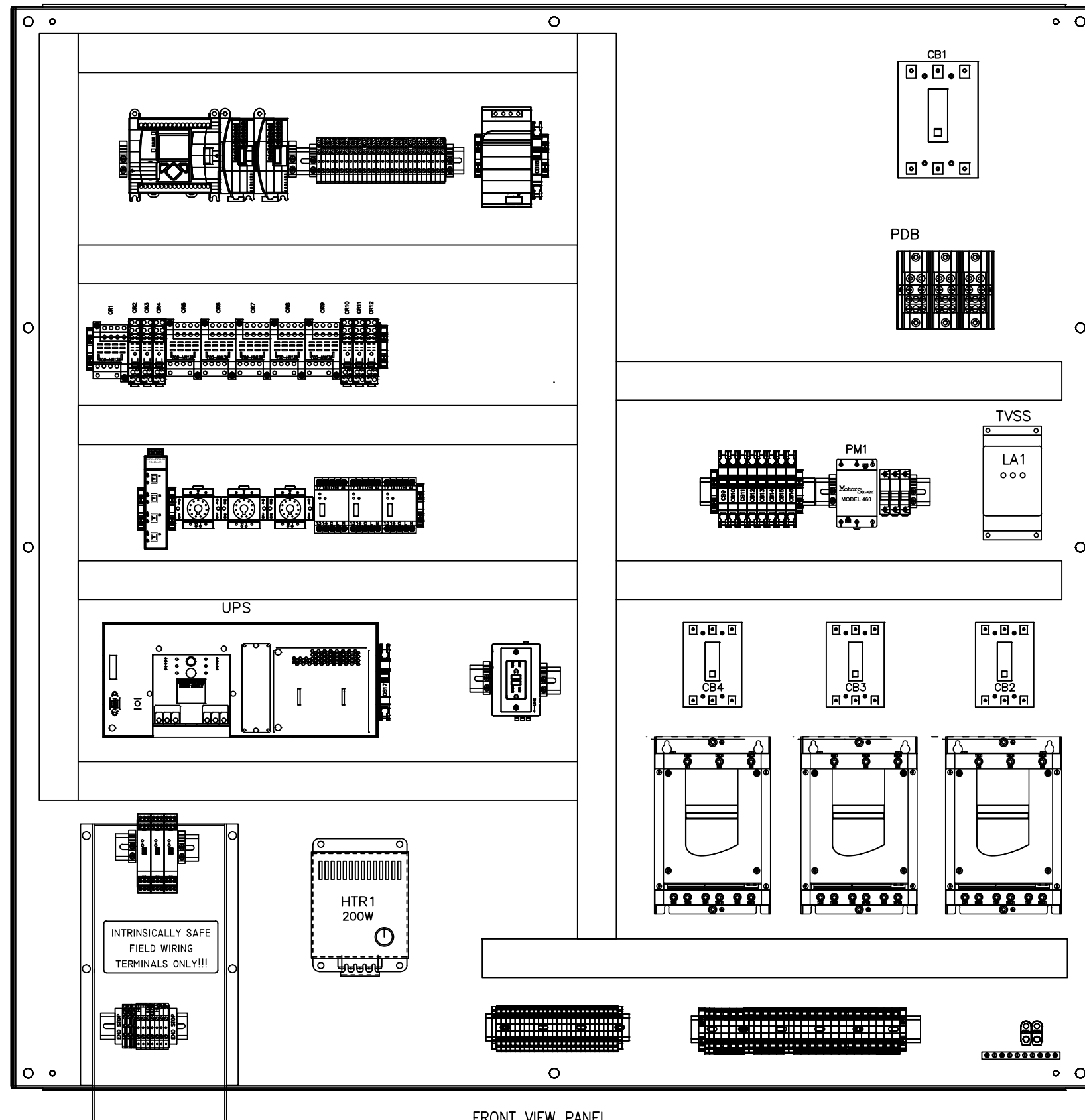
FRONT VIEW PANEL (DOOR/SWING OUT PANEL REMOVED)
