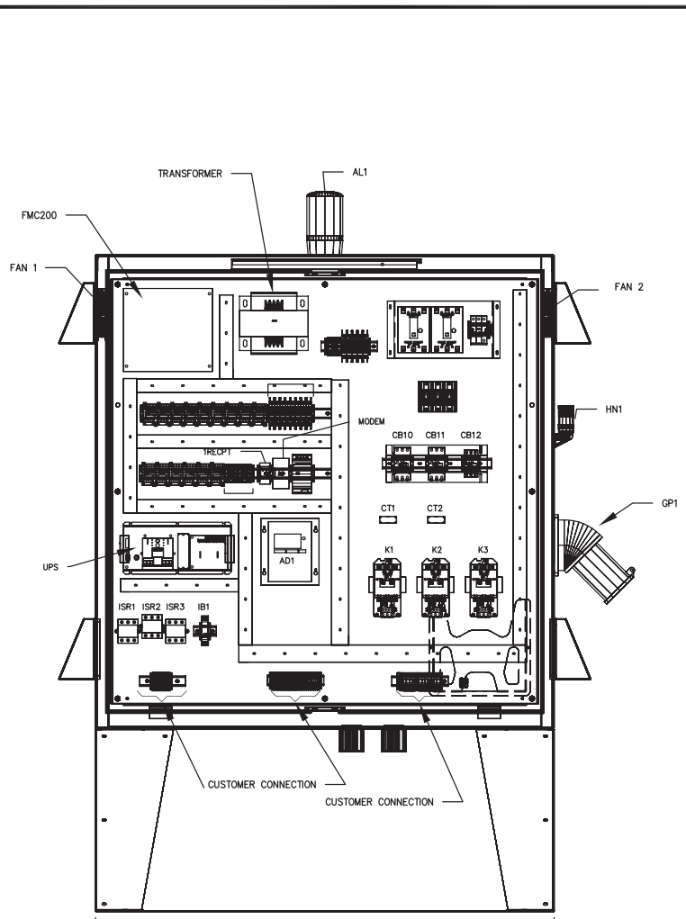
FRONT VIEW (DOORS/SWING OUT PANELS REMOVED)
