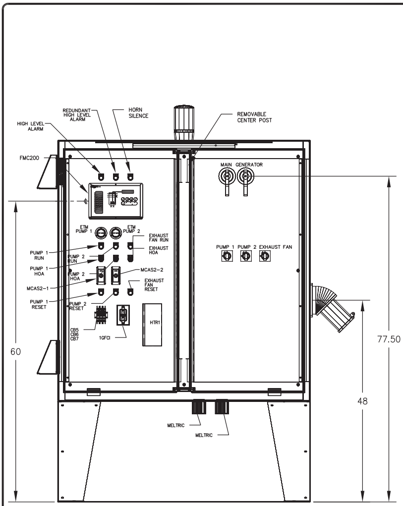
FRONT VIEW SWING PANELS (DOORS REMOVED)
