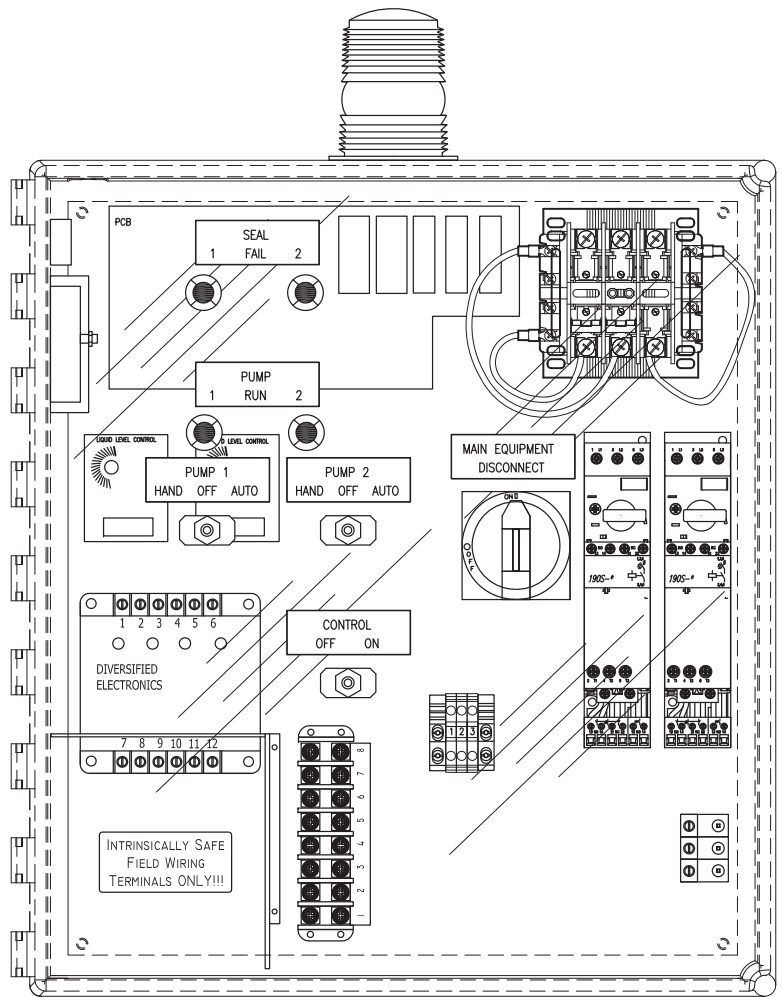
18 x 16 x 10 ENCLOSURE WITH OUTER DOOR REMOVED LEXAN INNER DOOR
