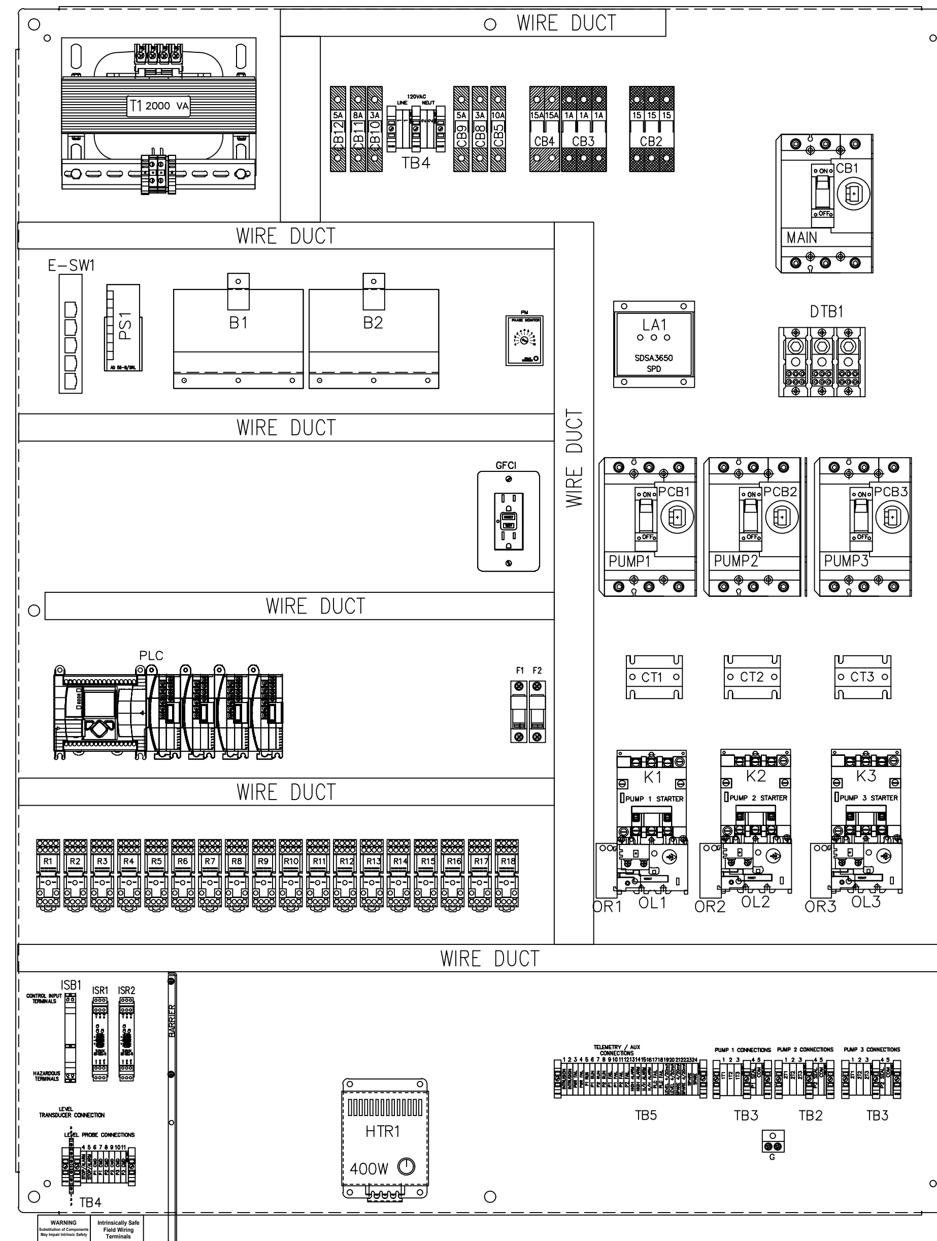
FRONT VIEW SUBPANEL
