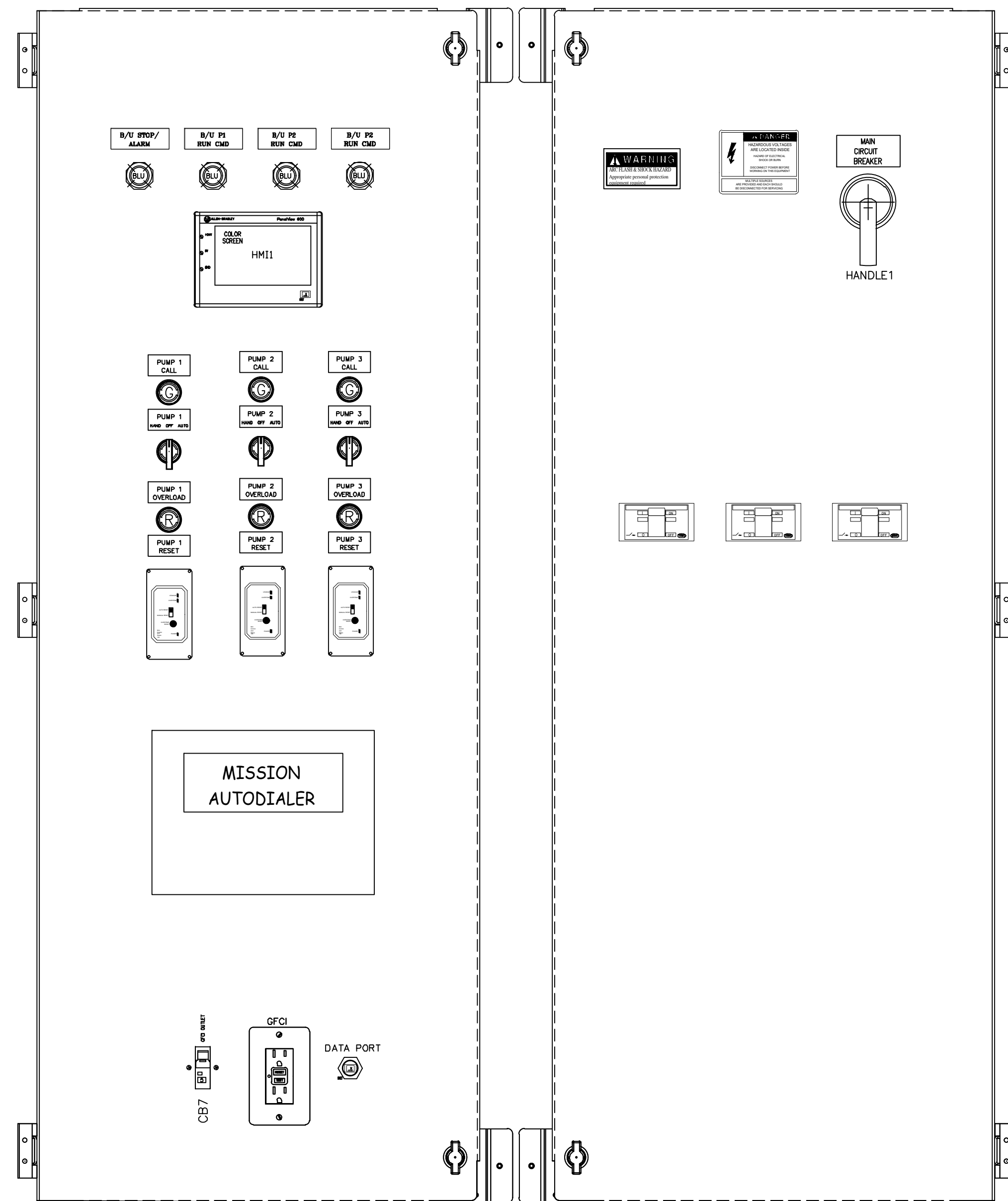
FRONT VIEW SWING PANELS
