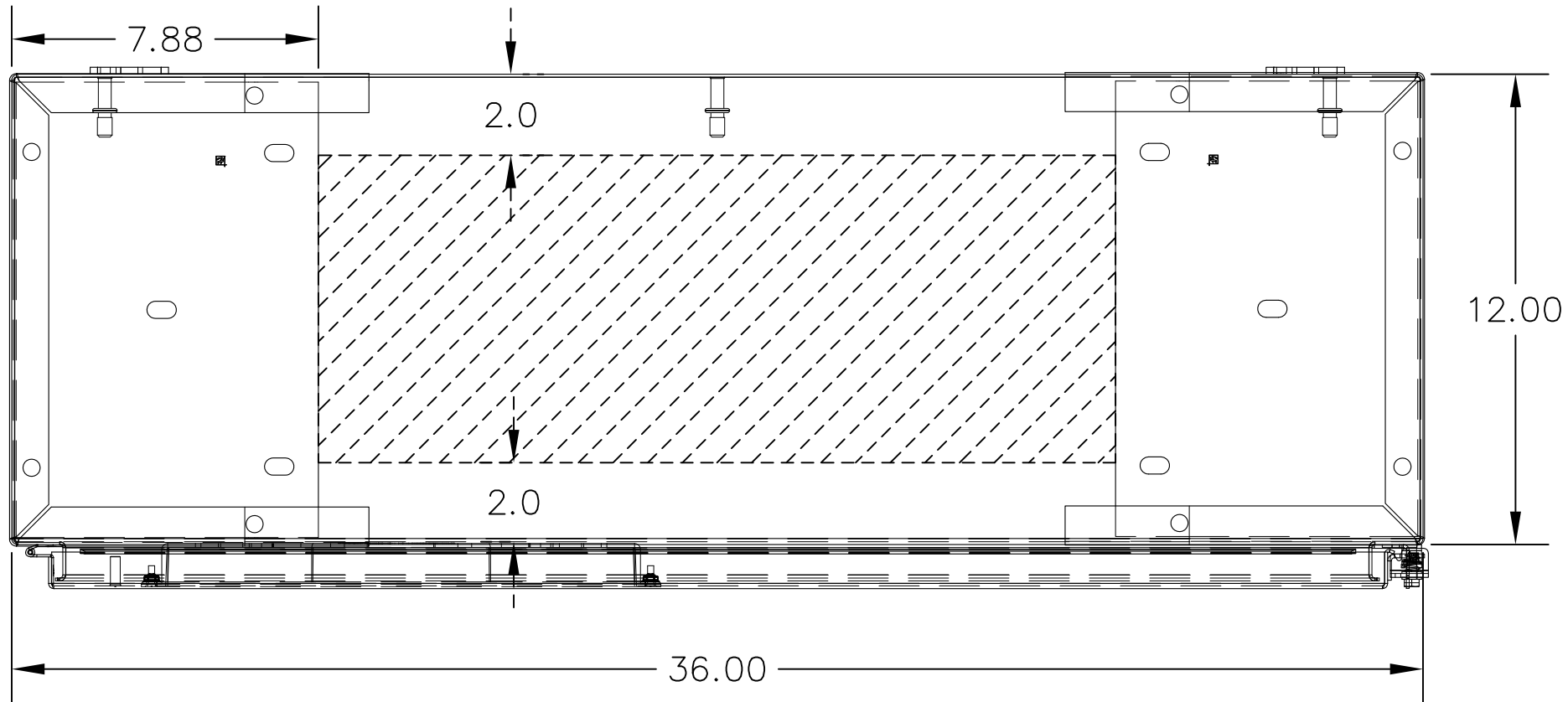
36"W X 12" D CONTROL PANEL WITH FLOOR STAND KIT
