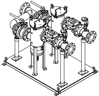
ISO VIEW SCALE 1 / 12
