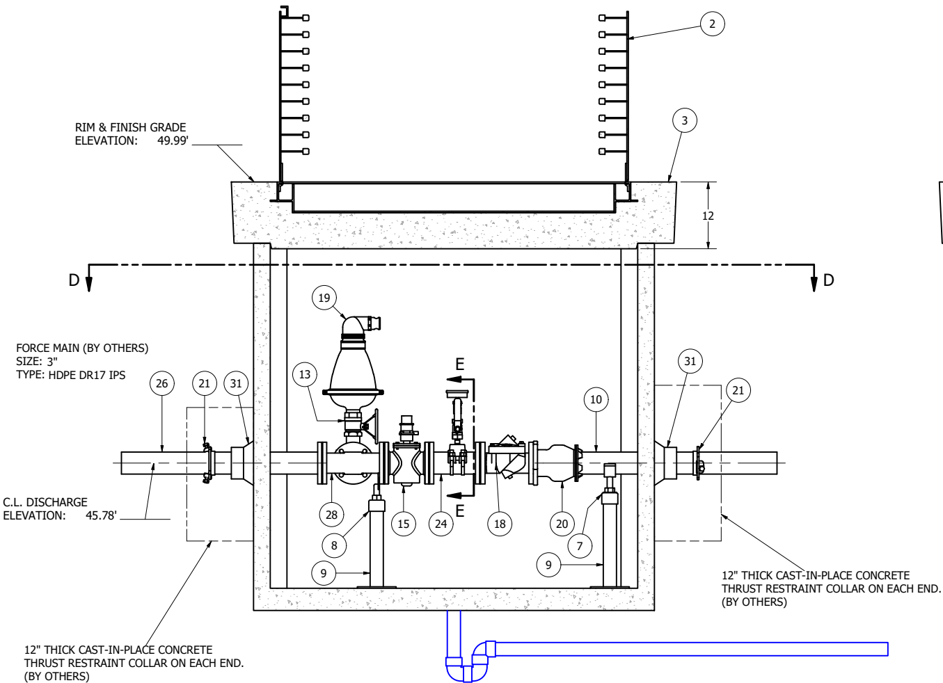
SECTION C-C SCALE 1 / 12
