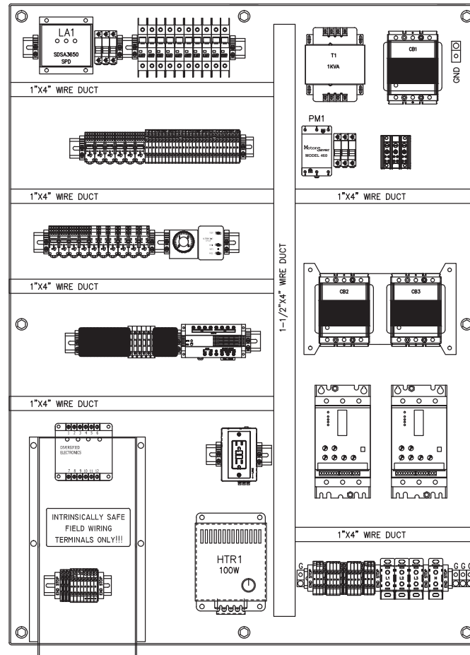
BACK PANEL LAYOUT
