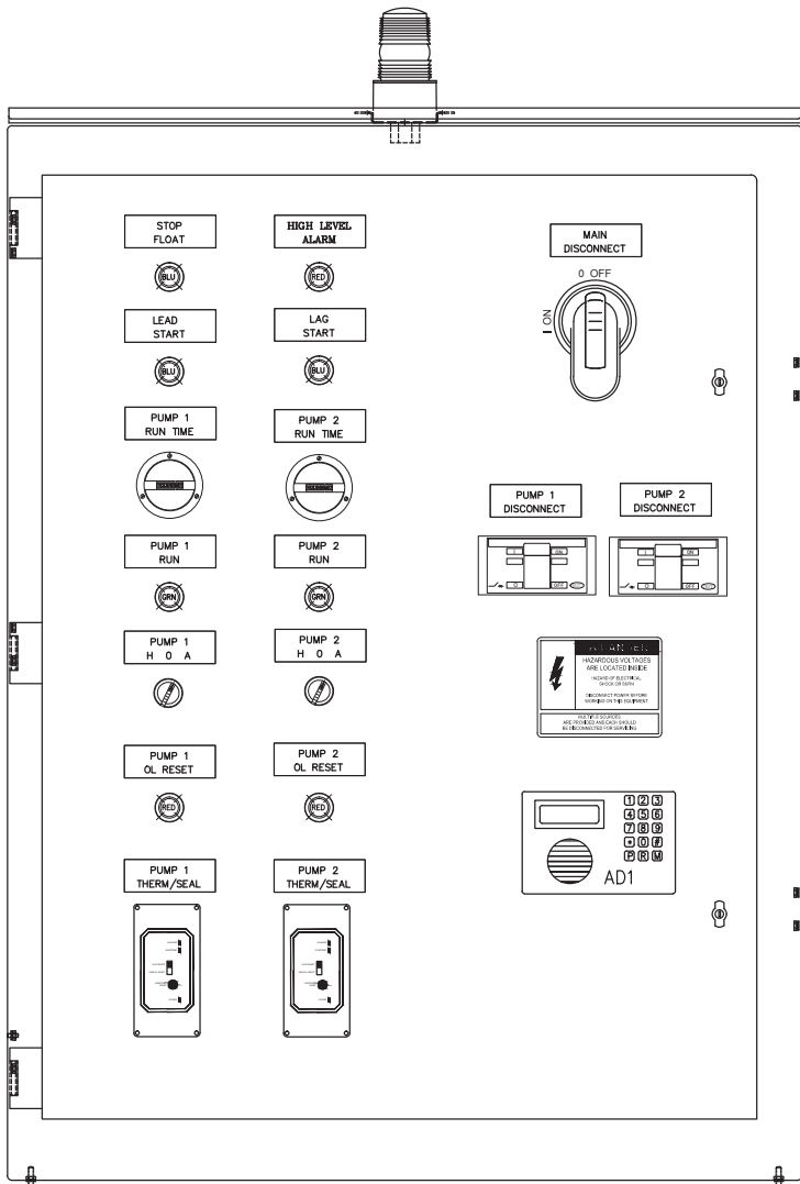
PUMP CONTROL PANEL
