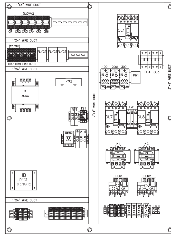
FRONT VIEW PANEL (DOOR/SWING OUT PANEL REMOVED)
