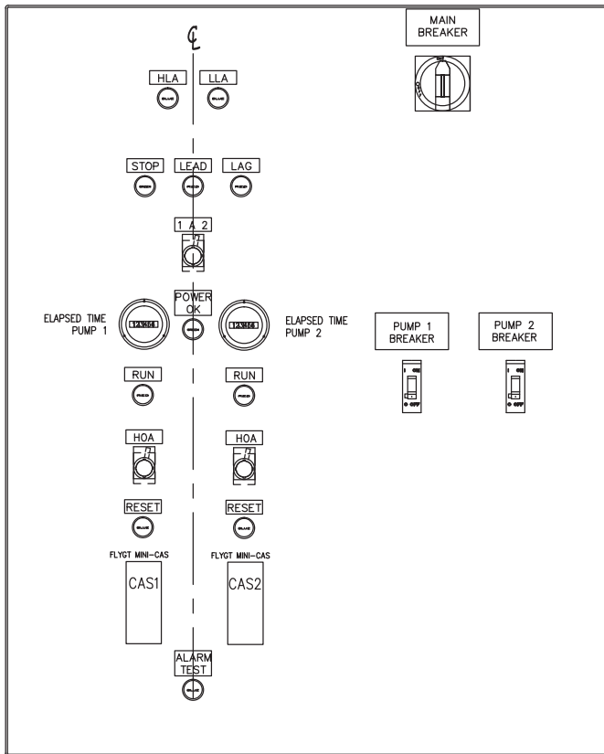
FRONT VIEW SWING PANEL (DOOR REMOVED)
