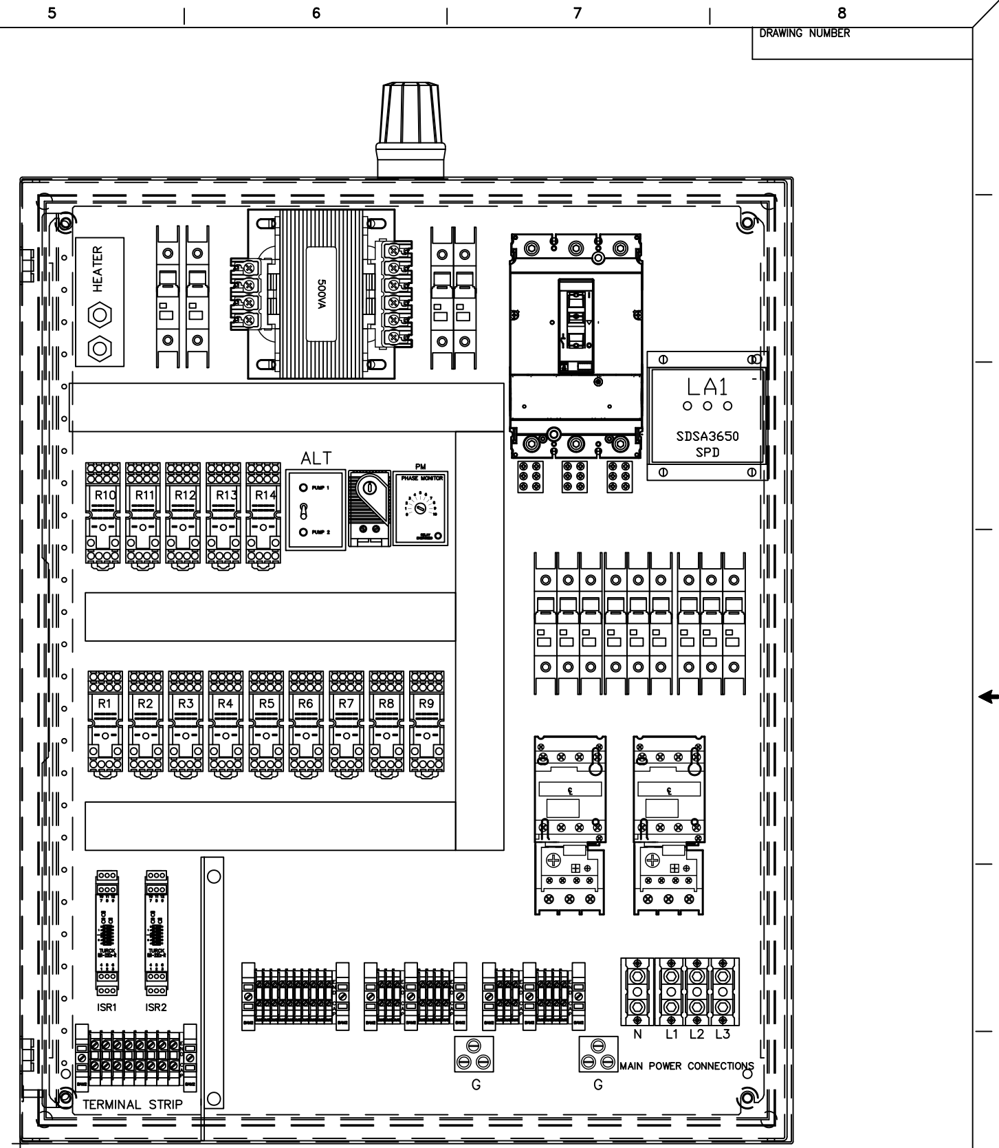
BACK PLATE VIEW
