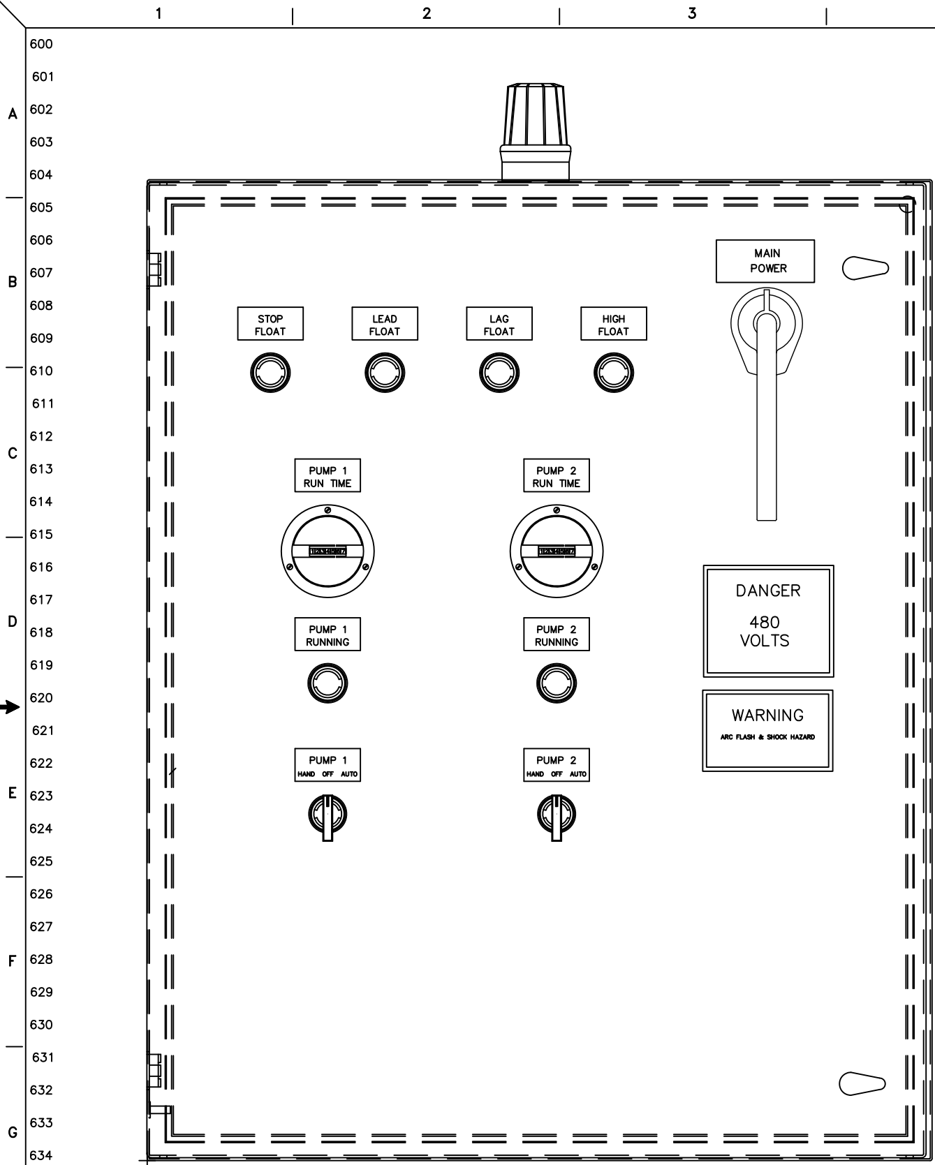
DEAD FRONT VIEW
