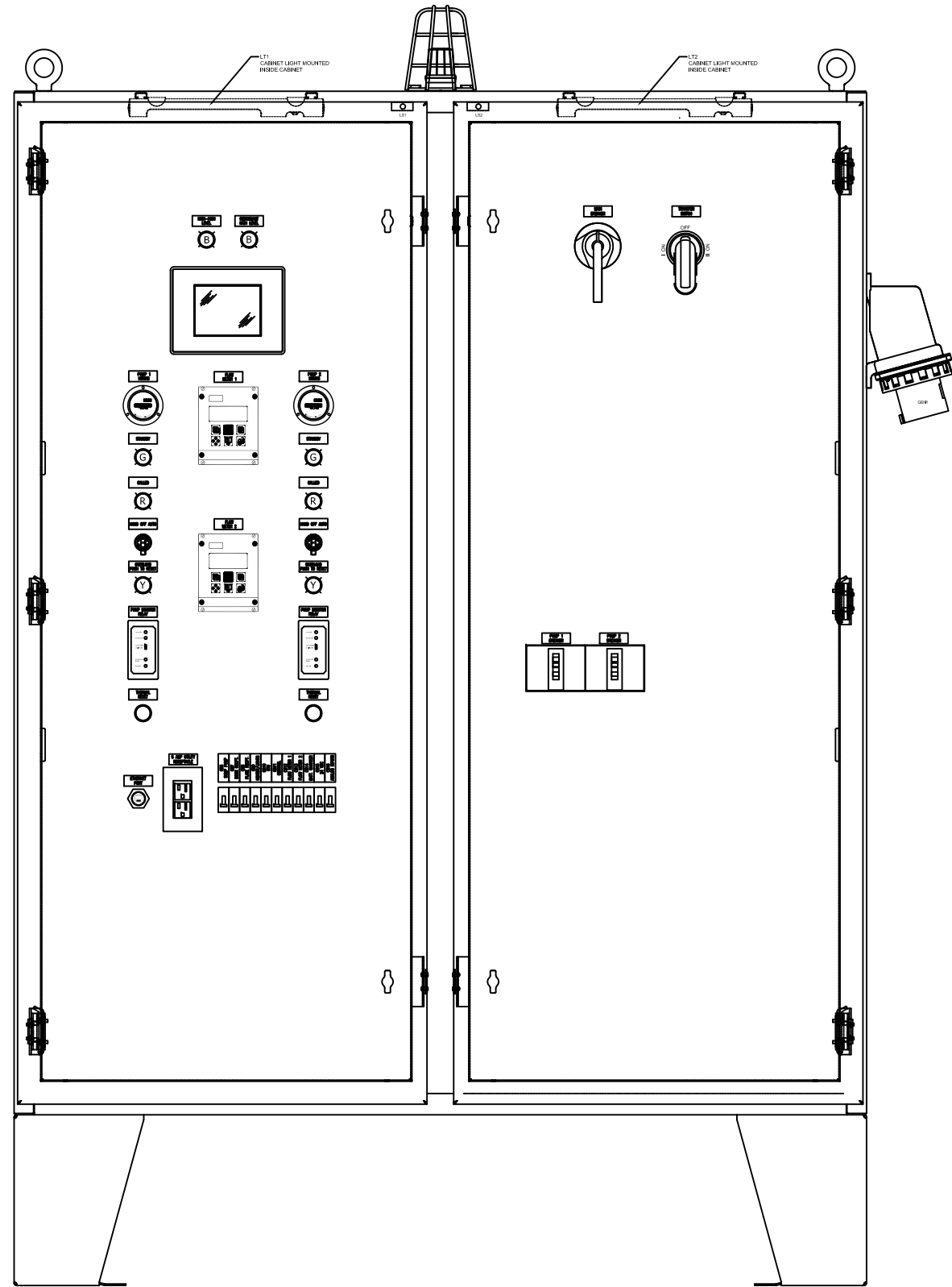
INNER DOORS
