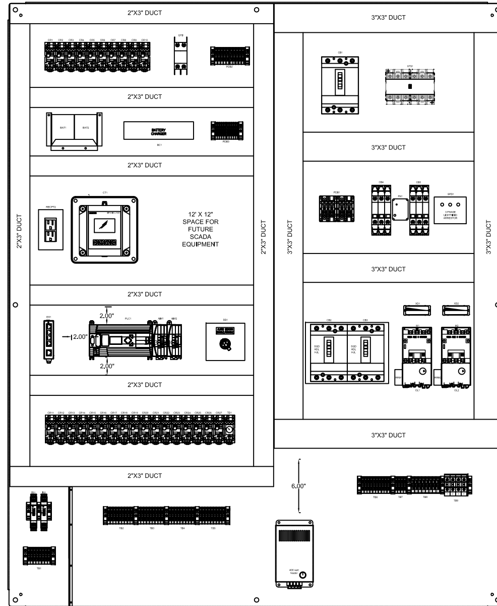
BACK PLATE
