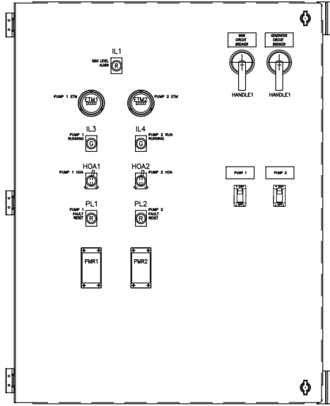
FRONT VIEW INNER DOOR
