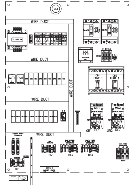
FRONT VIEW SUBPANEL
