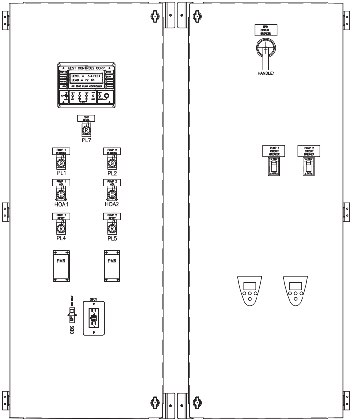
FRONT VIEW SWING PANELS
