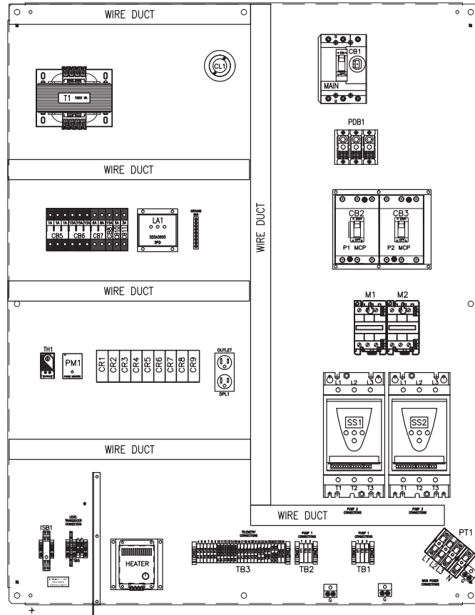
FRONT VIEW SUBPANEL
