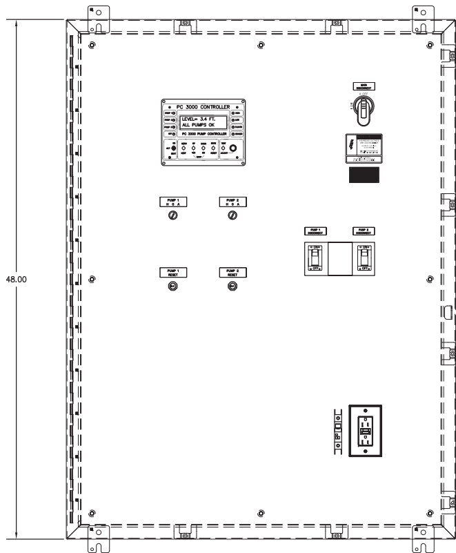
PUMP CONTROL PANEL 48" H x 36" W x 10" D FRONT VIEW WITH OUTER DOOR REMOVED
