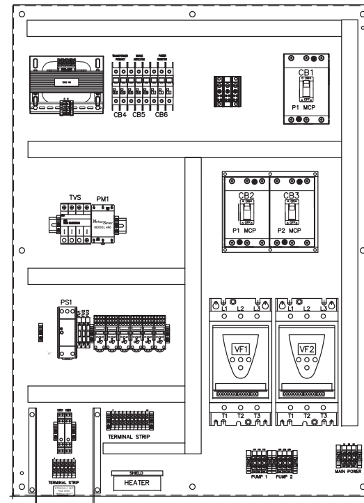
PUMP CONTROL PANEL BACK PANEL VIEW
