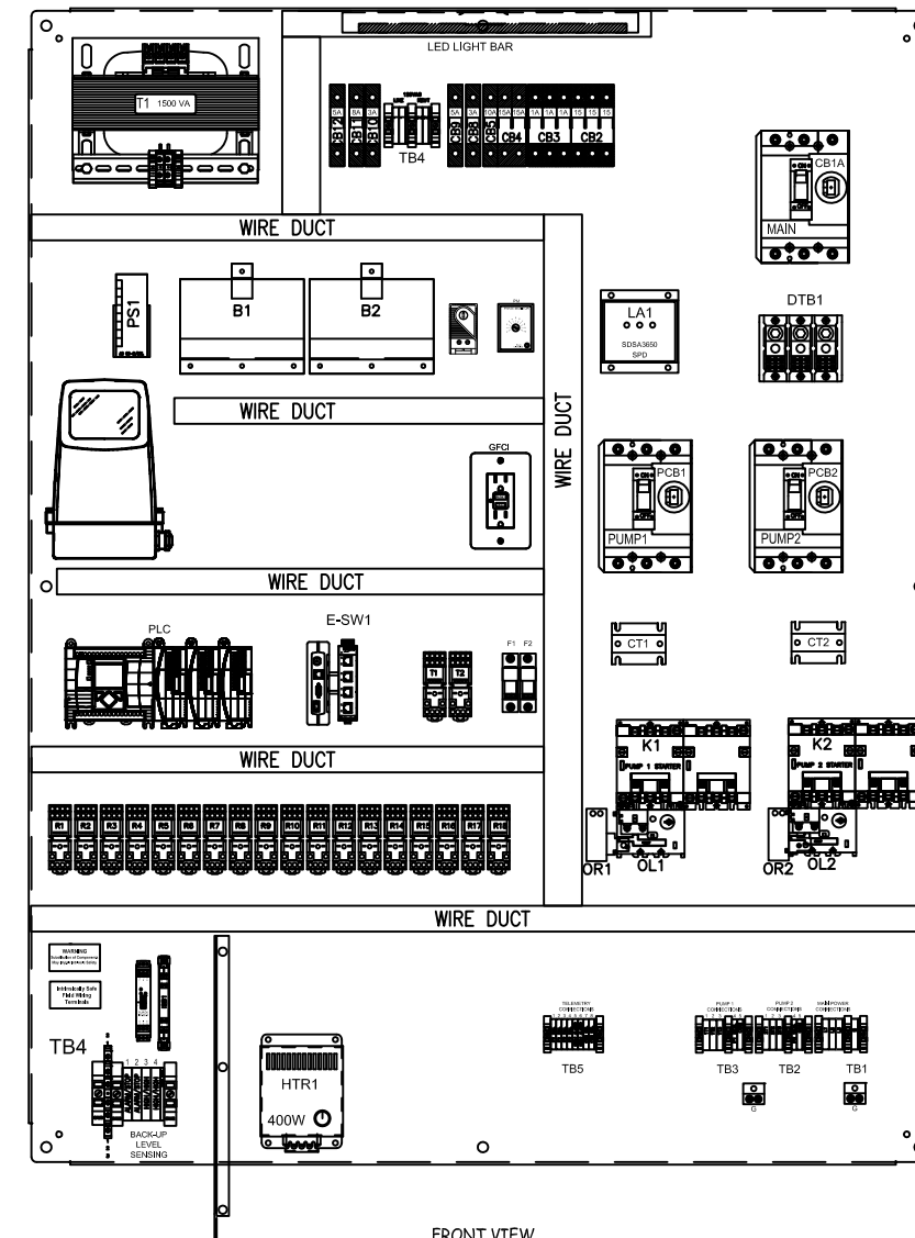
FRONT VIEW SUBPANEL
