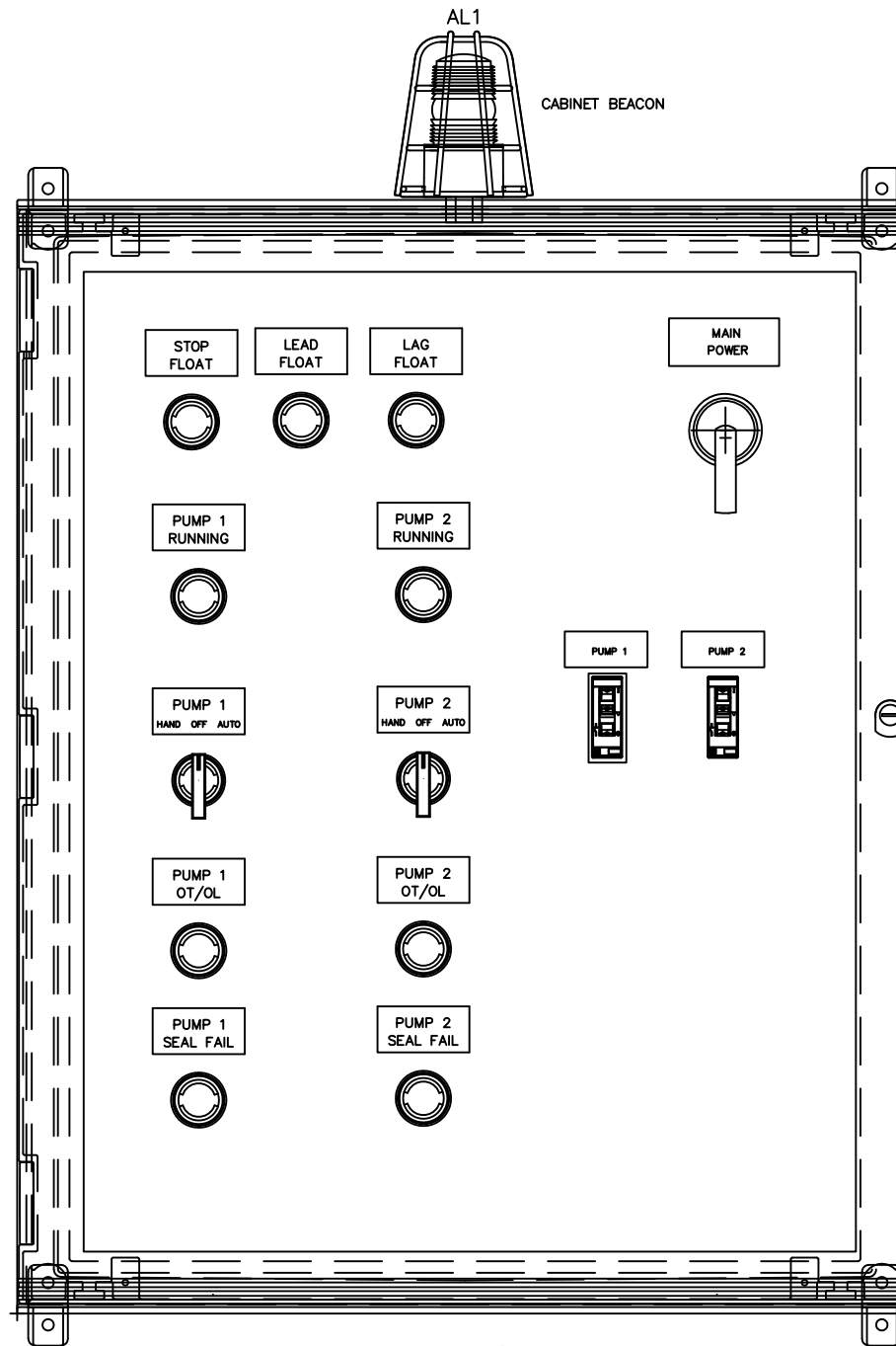
FRONT VIEW INNER DOOR
