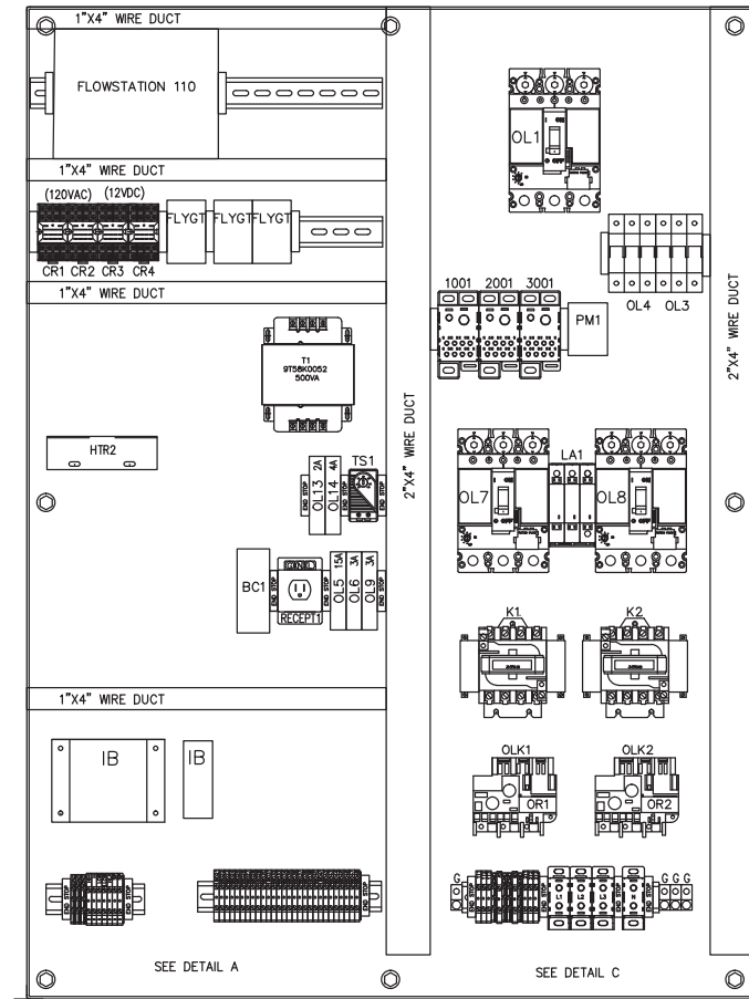
FRONT VIEW PANEL (DOOR/SWING OUT PANEL REMOVED)
