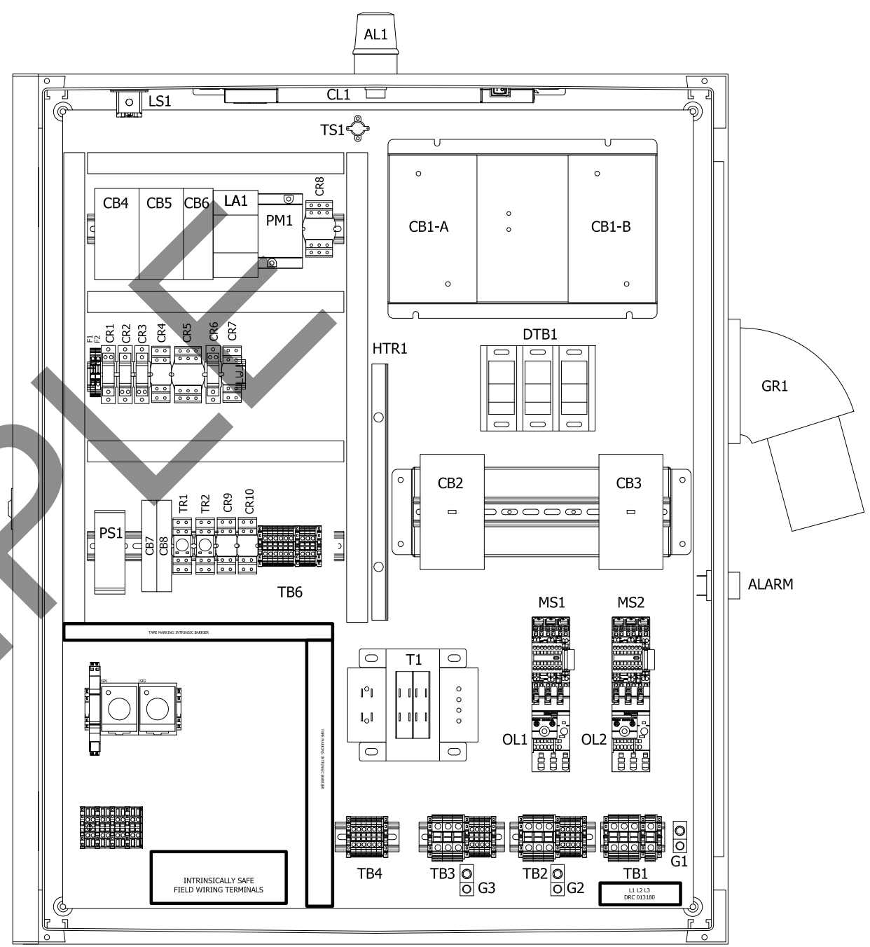
BACK PANEL VIEW
