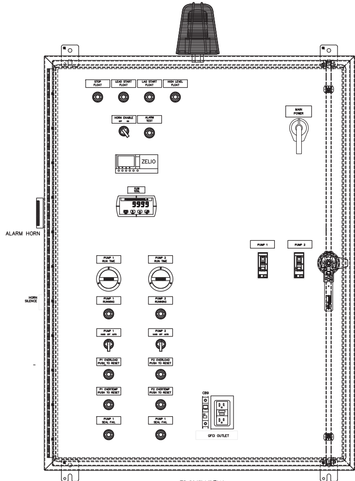
FRONT VIEW INNER DOOR
