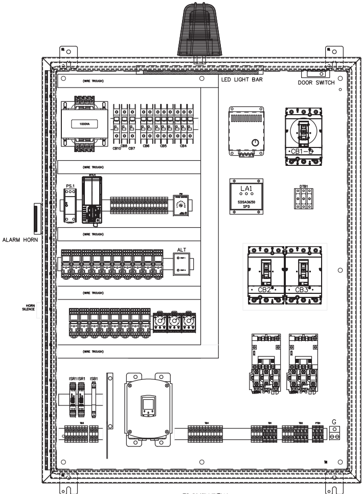
FRONT VIEW BACKPLATE
