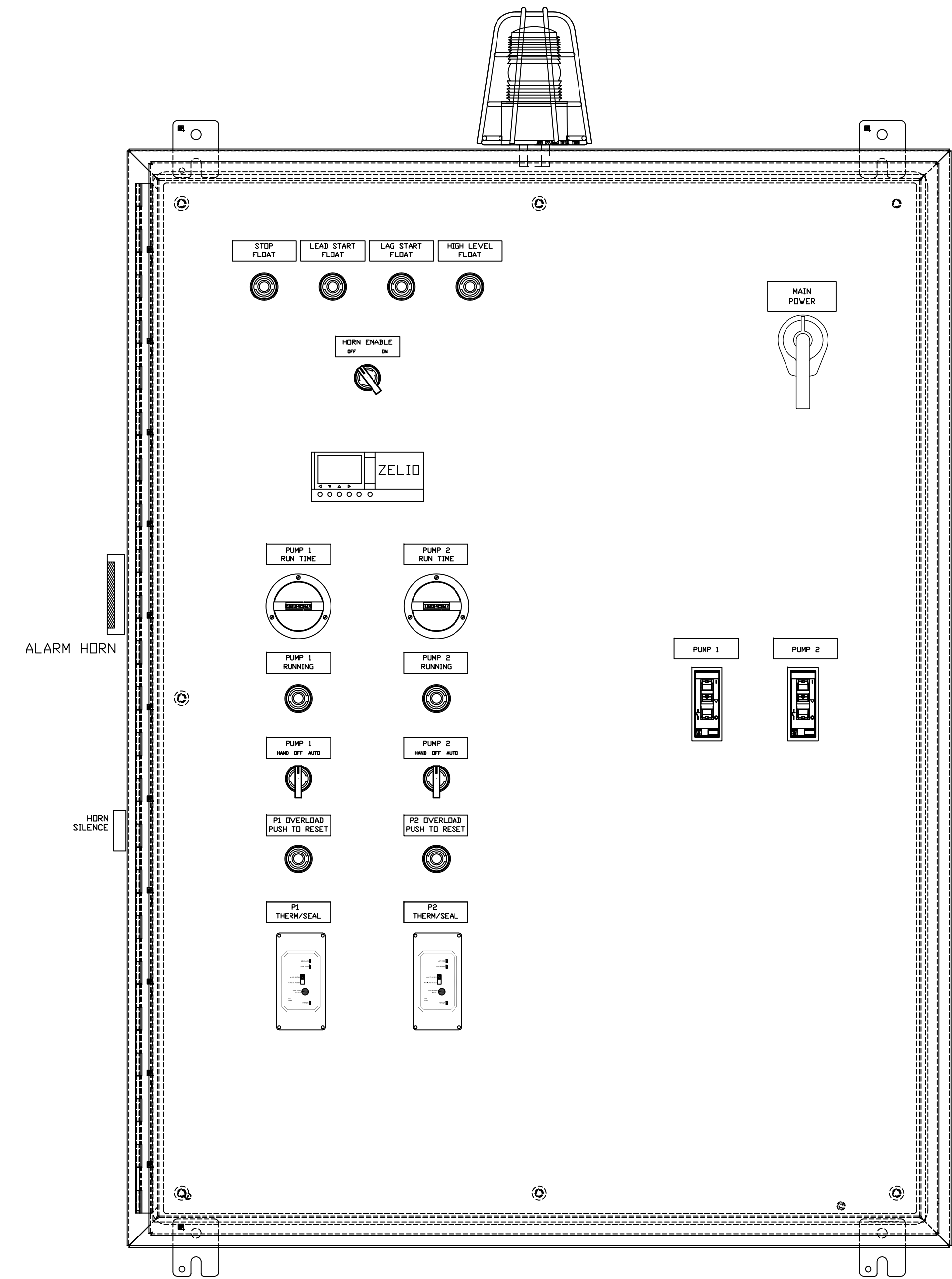
INNER DOOR VIEW
