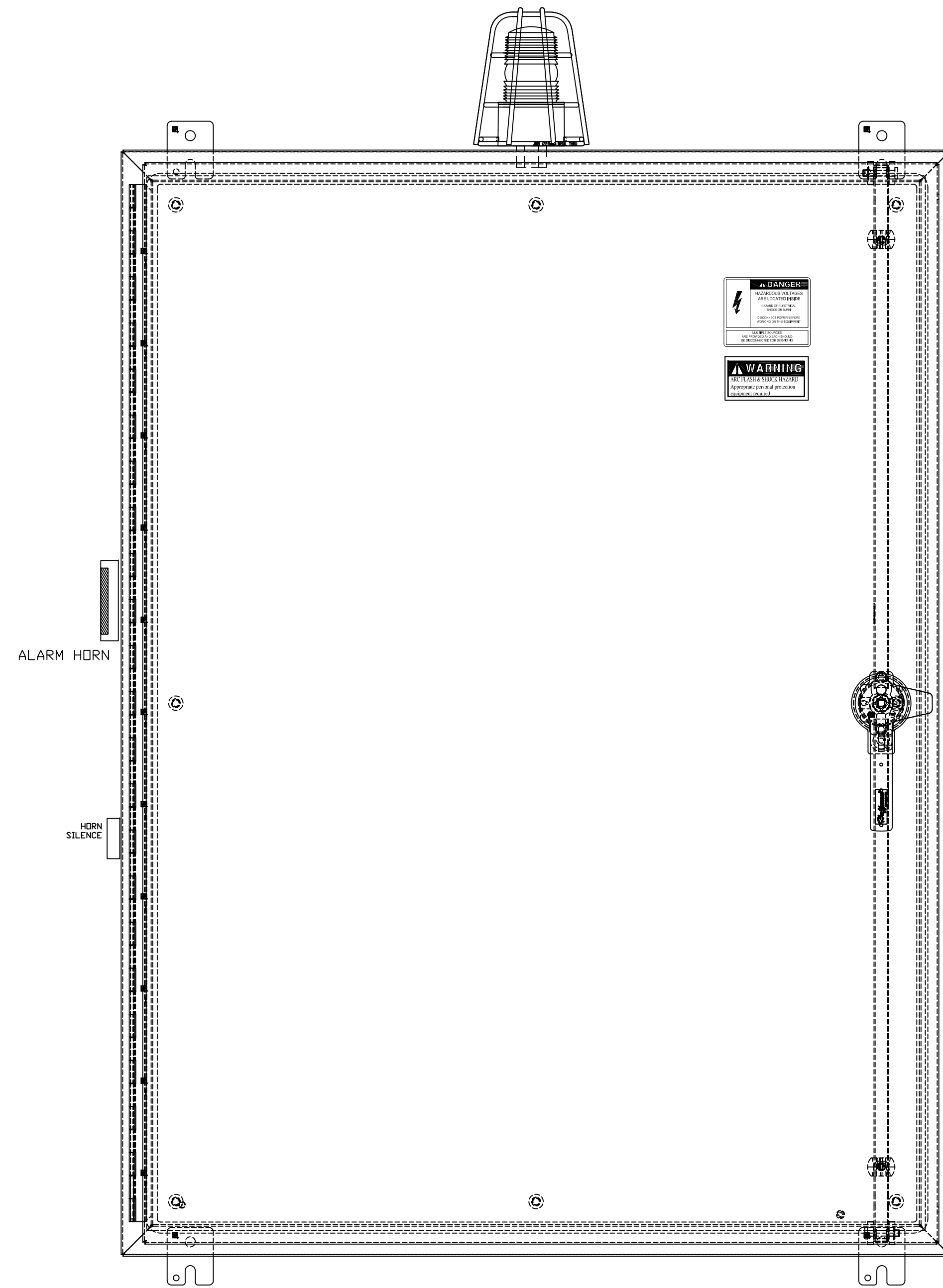
OUTER DOOR VIEW
