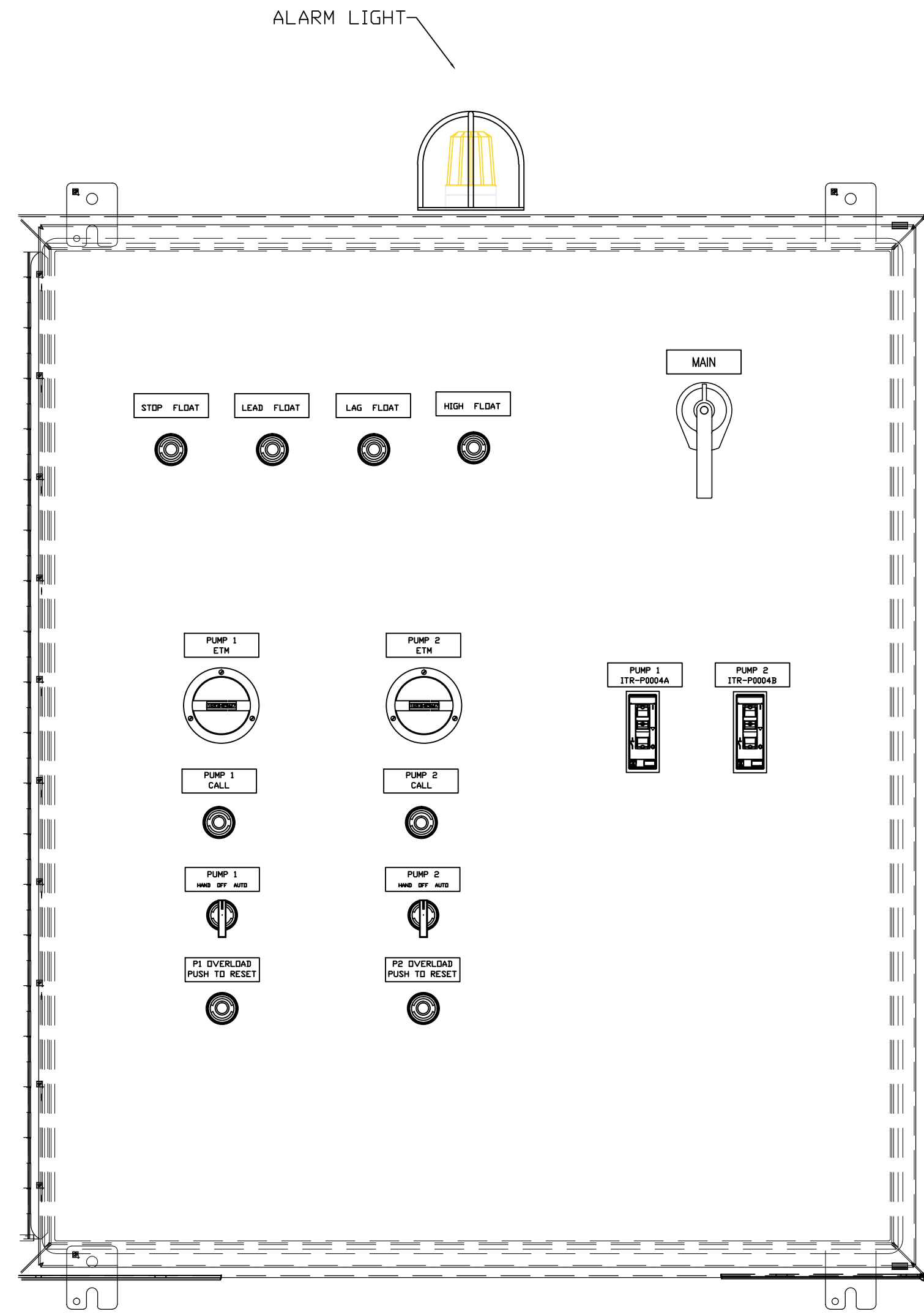
DEADFRONT VIEW
