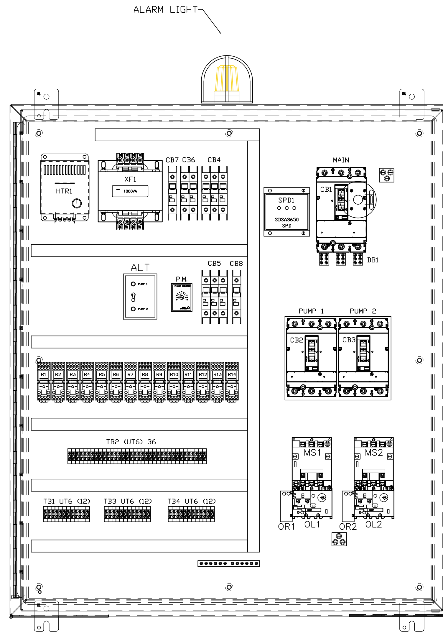
BACKPLATE VIEW
