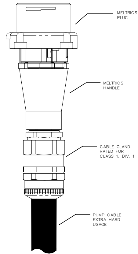
MELTRIC PLUG DETAIL
