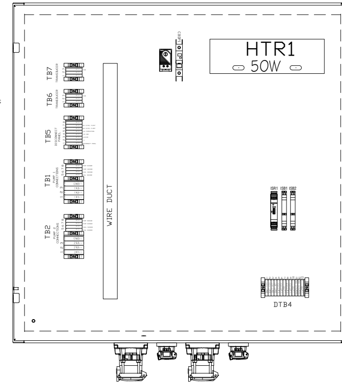
BACKPLATE VIEW
