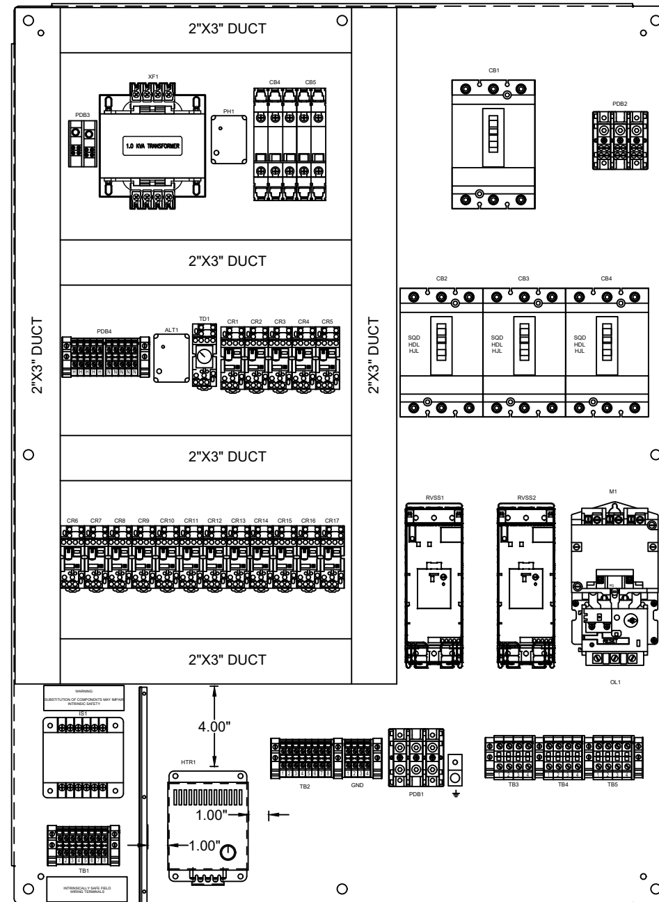
BACK PLATE
