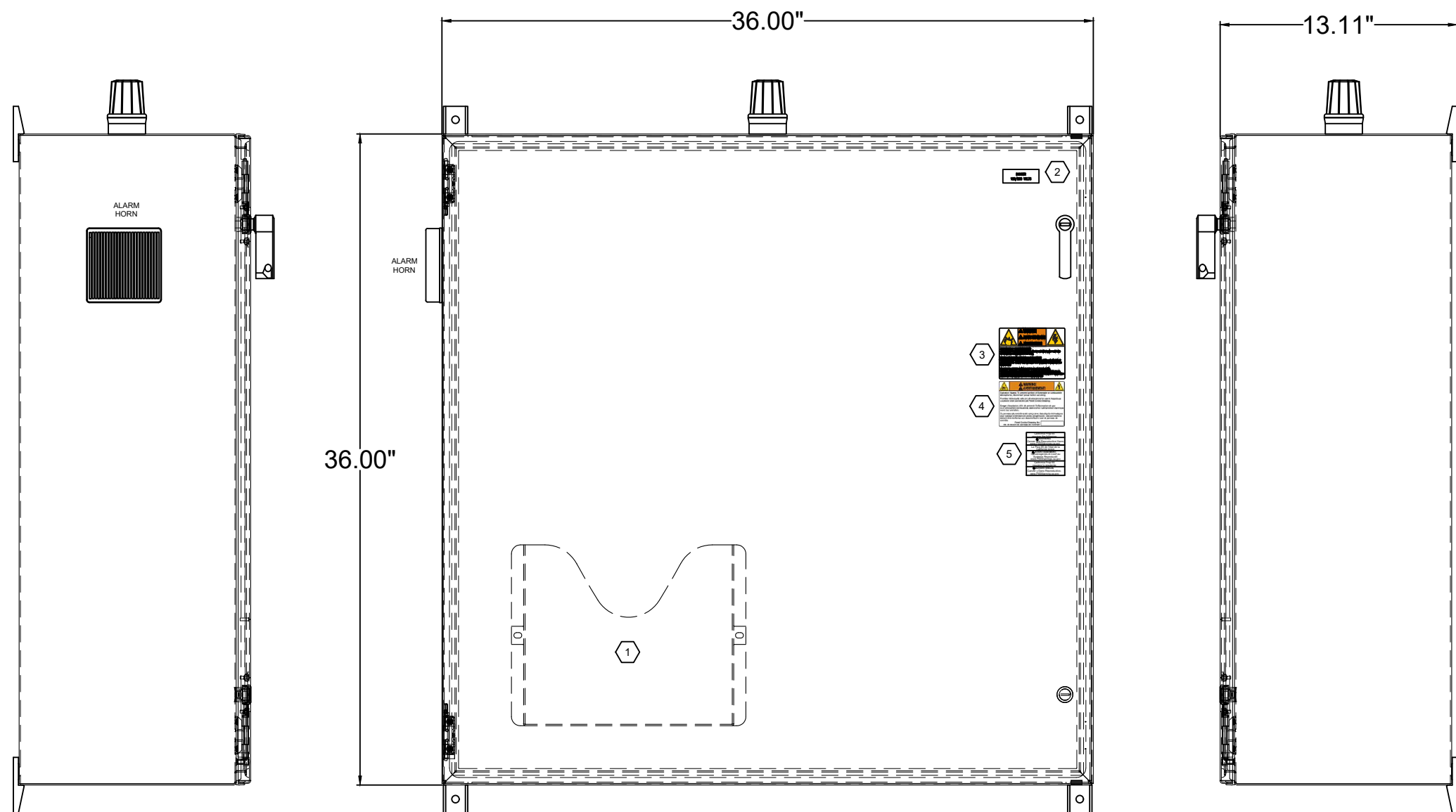
LEFT SIDE EXTERIOR VIEW
