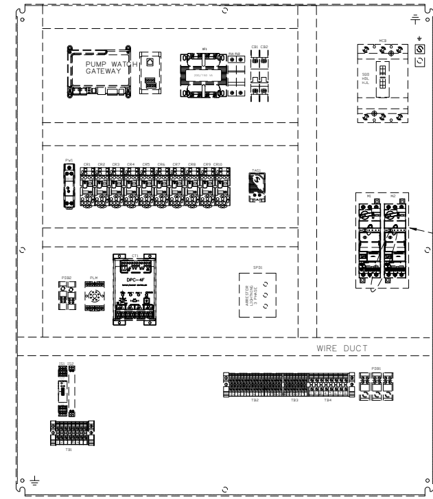
BACK PLATE
