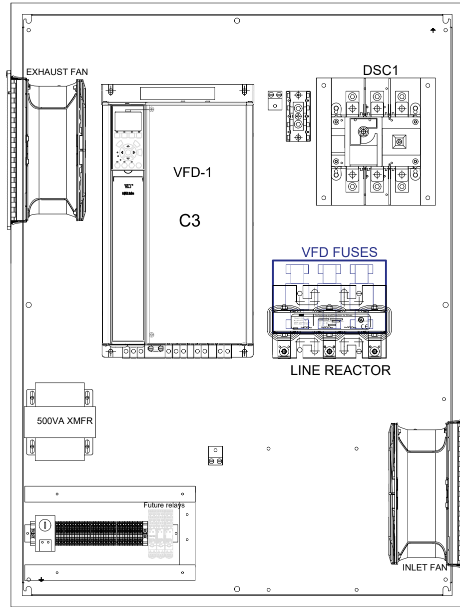
INSIDE VIEW
