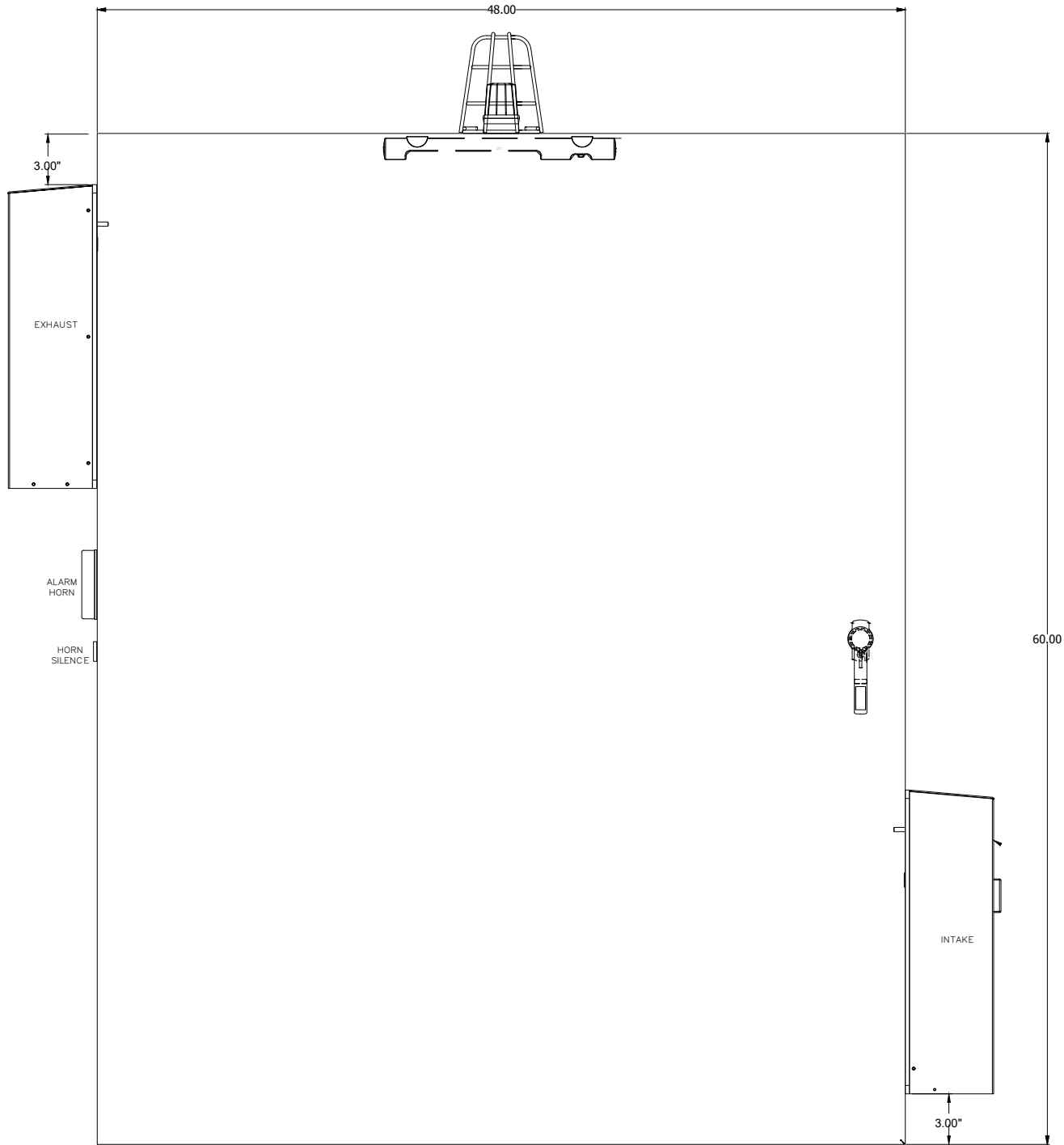
FRONT EXTERIOR VIEW (60"X48"X18", NEMA TYPE 3R SS)
