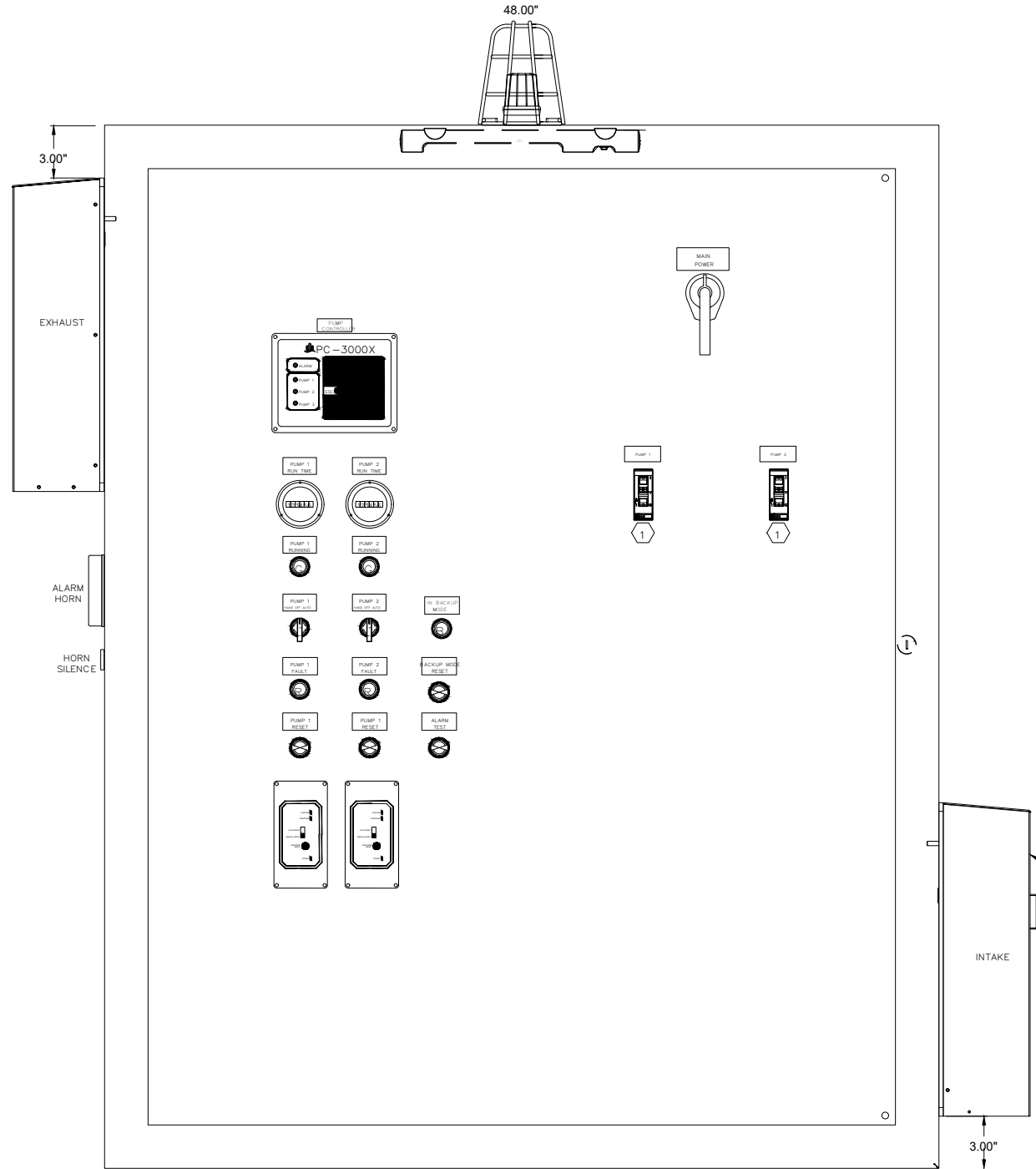
INNER DOOR VIEW (SHOWN WITH OUTER DOOR REMOVED)
