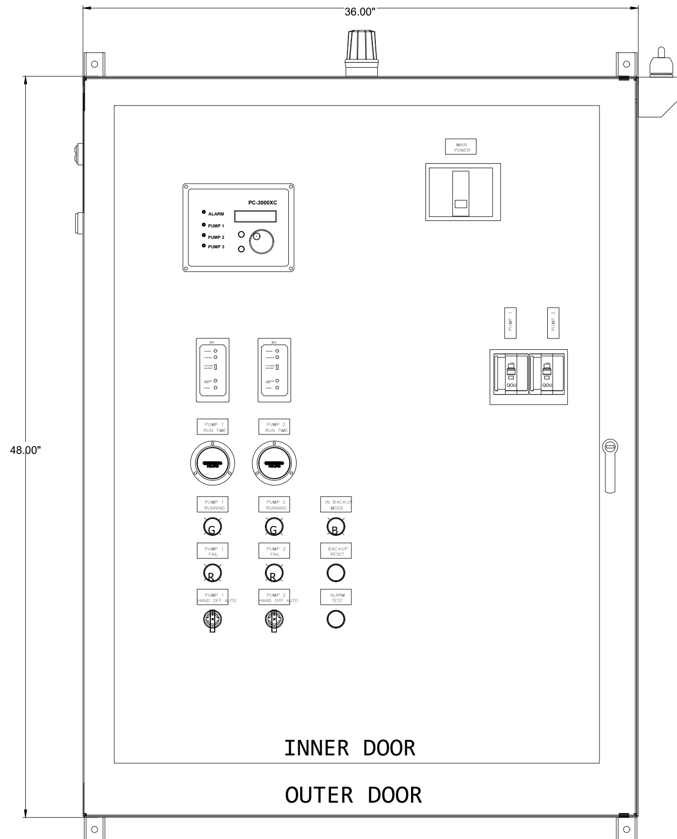
INNER DOOR HOFFMAN PAINTED STEEL - CSD483612
