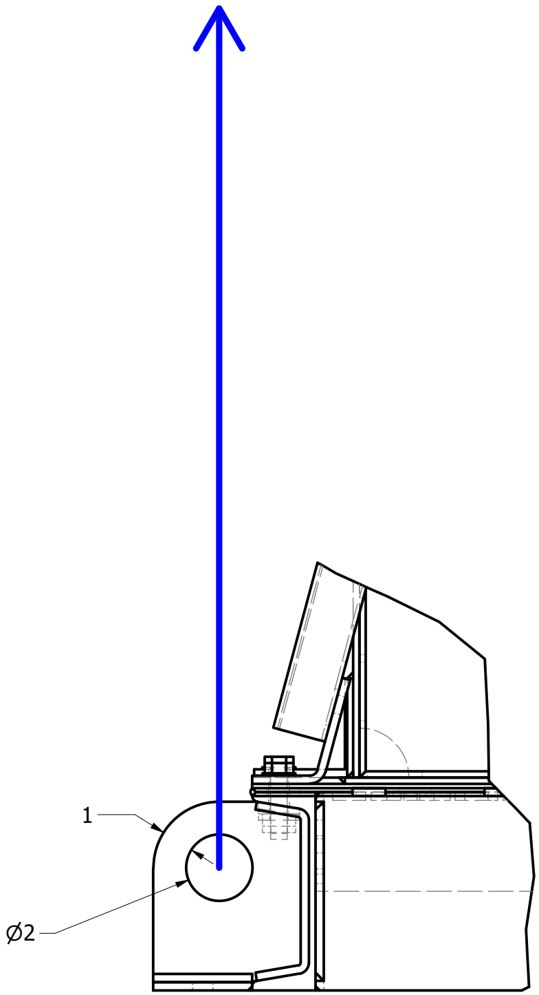
LIFTING EYE (TYP) DETAIL D SCALE 1 / 4
