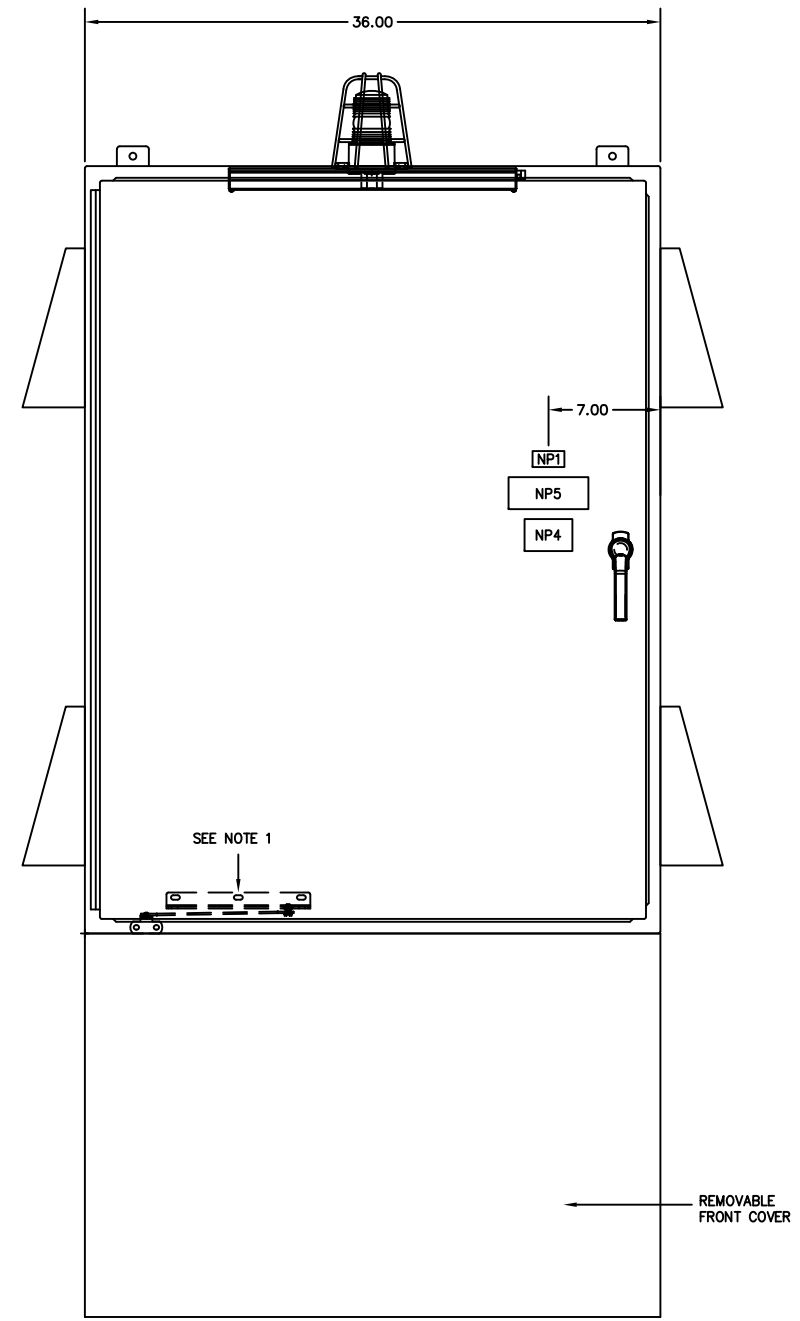
FRONT VIEW PANEL
