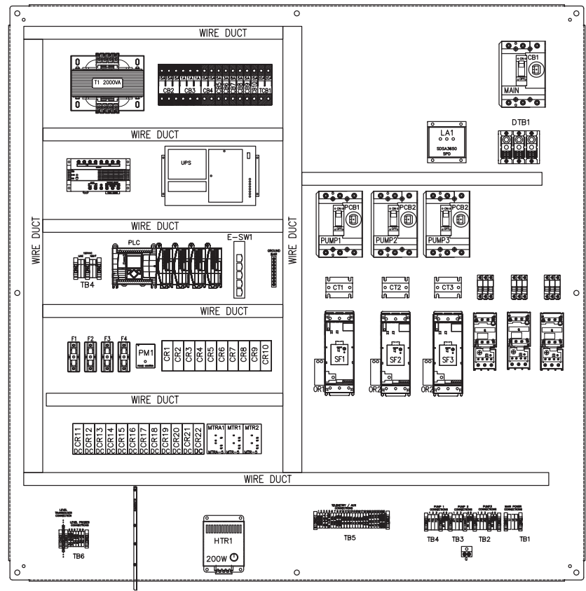
FRONT VIEW SUBPANEL
