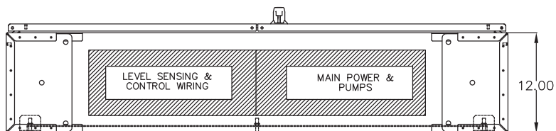
BOTTOM VIEW
