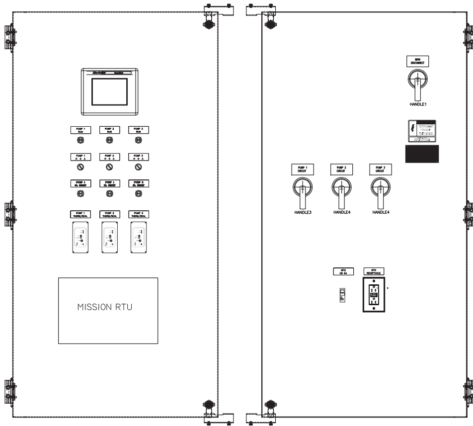
FRONT VIEW SWING PANELS
