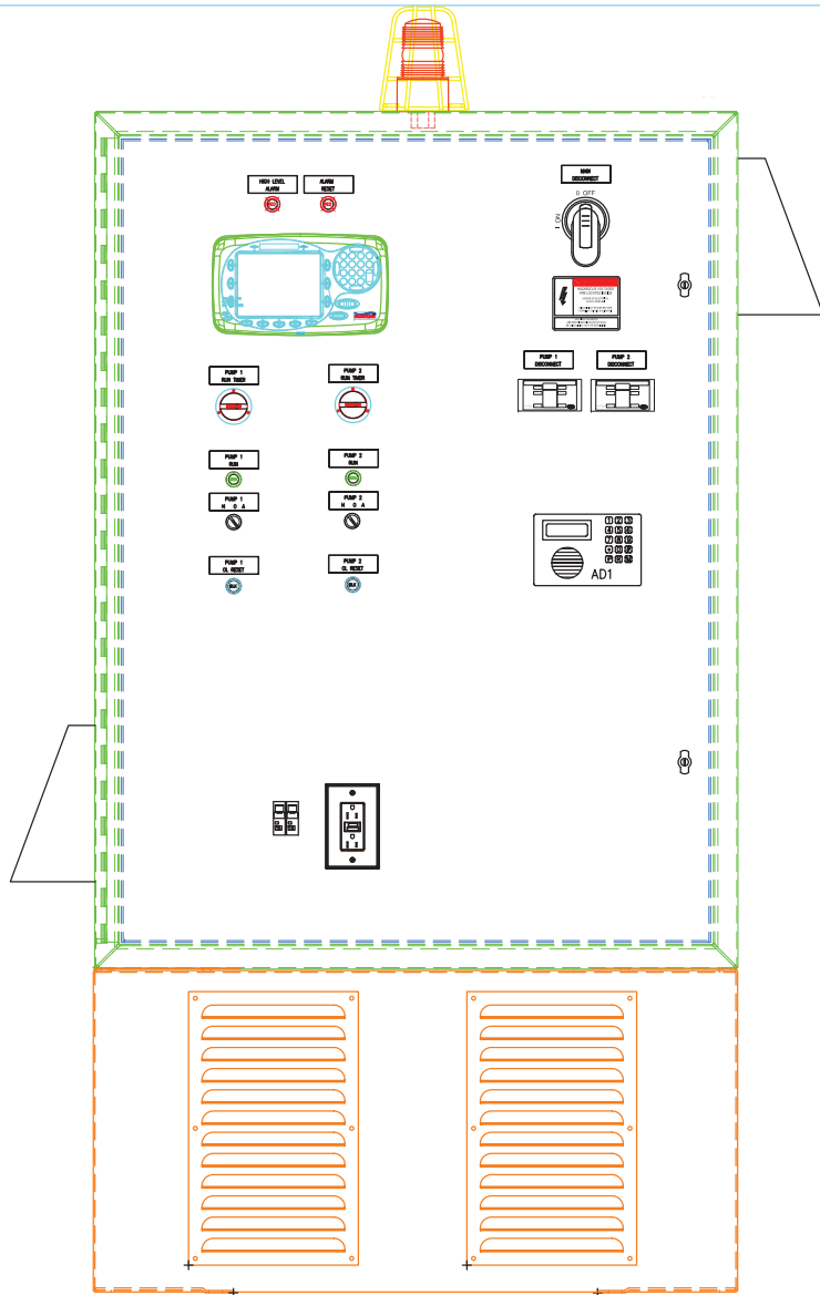
PUMP CONTROL PANEL 48"H x 36"W x 12"D 18" LEG KIT W/VENTED SKIRT FRONT VIEW WITH OUTER DOOR REMOVED
