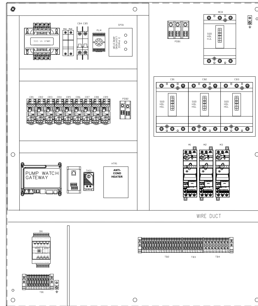
BACK PANEL
