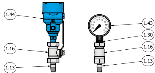
PRESSURE GAUGE & TRANSMITTER DETAIL DETAIL C SCALE 1 / 5
