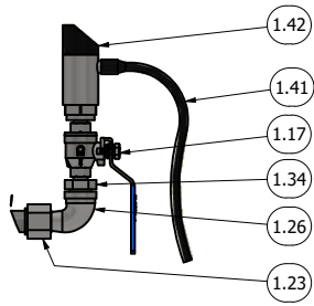
PRESSURE SWITCH DETAIL DETAIL B SCALE 1 / 4
