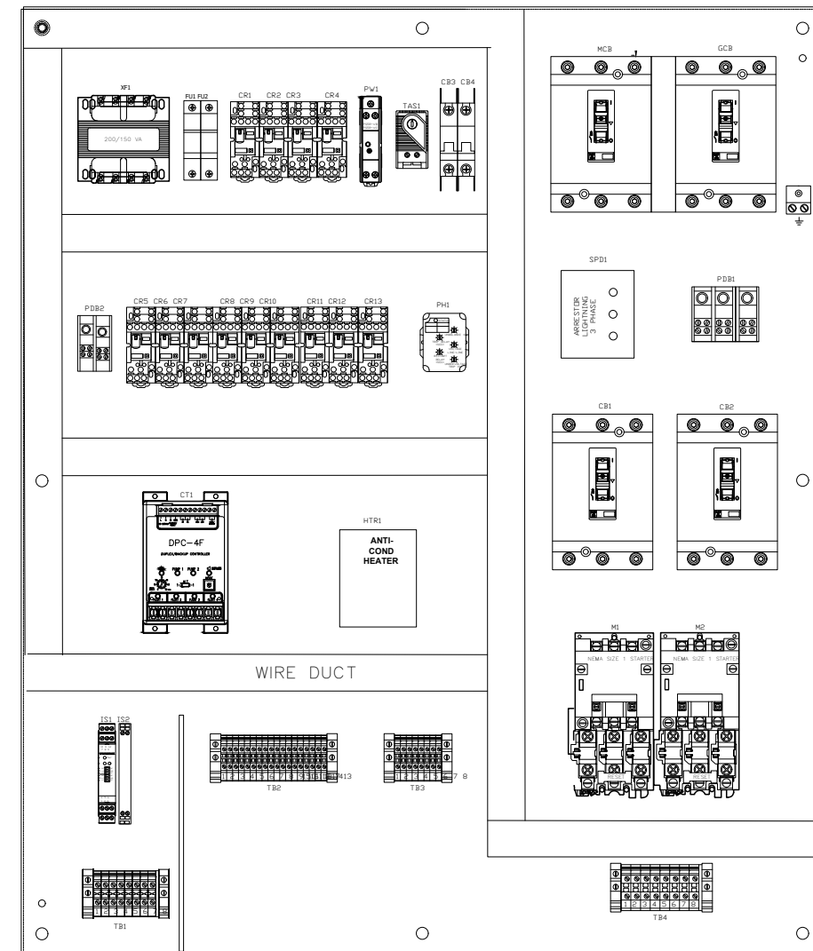
BACK PLATE
