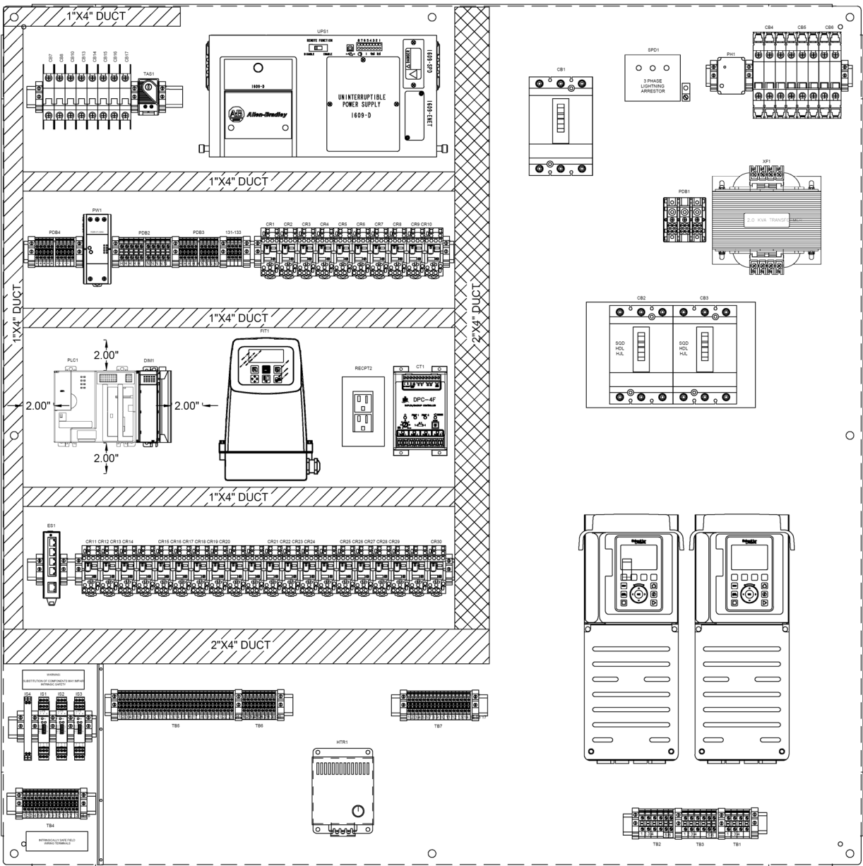
BACK PLATE
