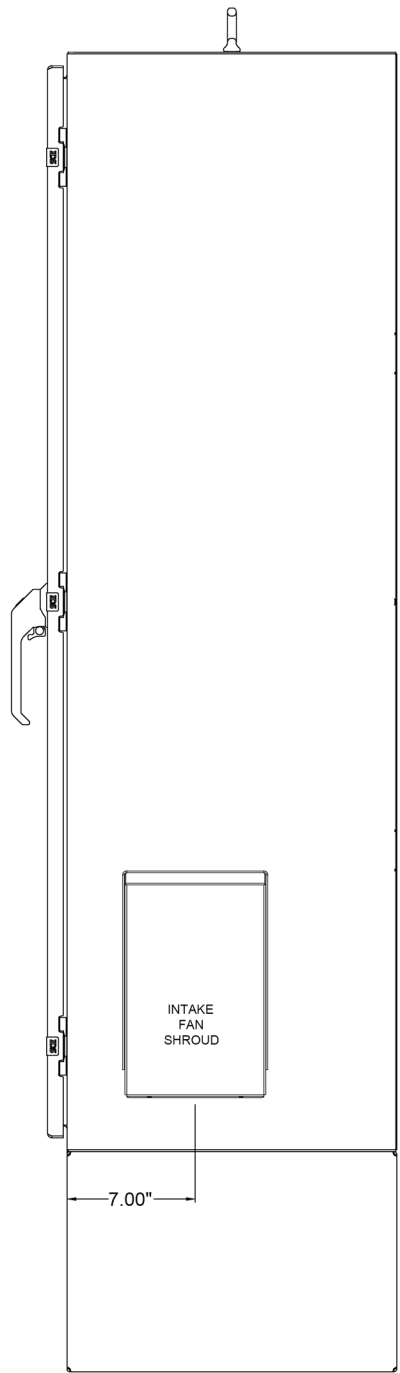
RIGHT SIDE EXTERIOR VIEW
