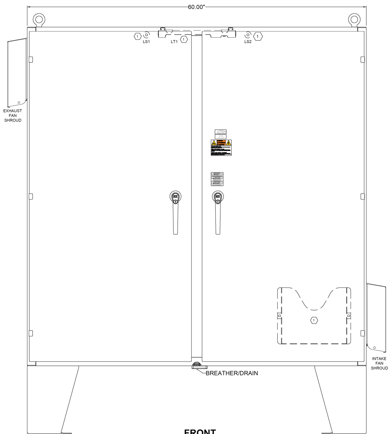
FRONT EXTERIOR VIEW (NEMA 4X)
