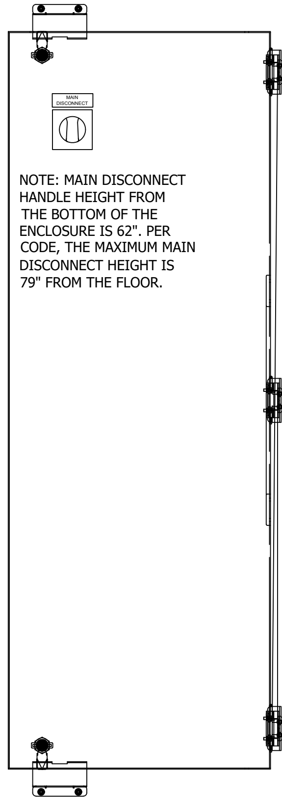
DEAD FRONT PANEL FRONT VIEW
