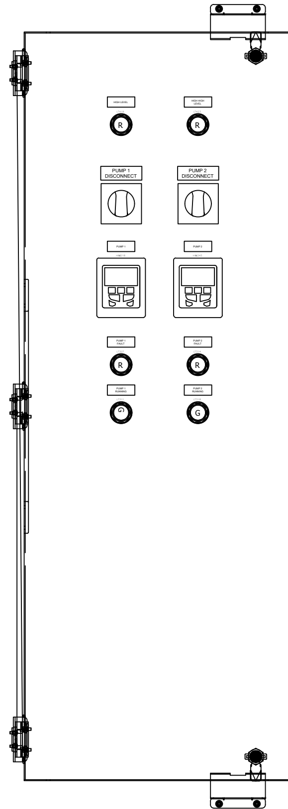
DEAD FRONT PANEL FRONT VIEW
